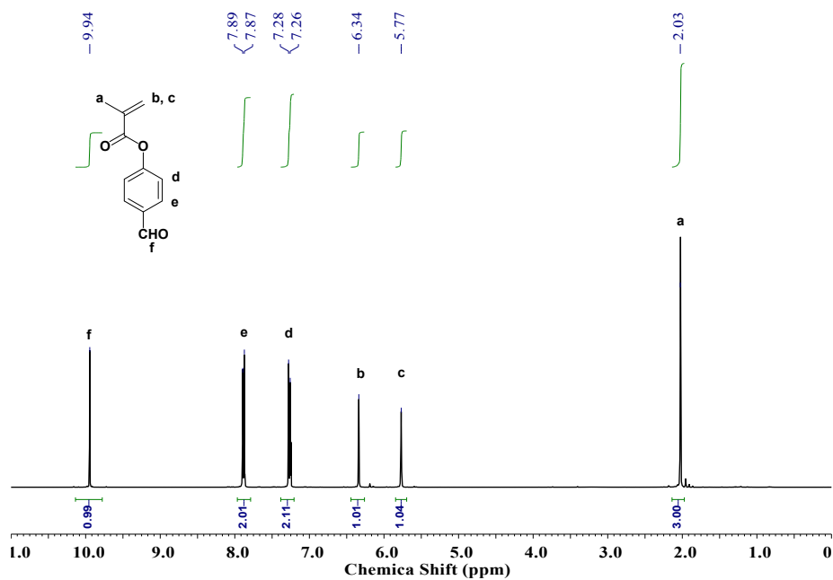
Fig. S1. ^1\text{H} NMR spectrum of FPMA in \text{CDCl}_3 .
