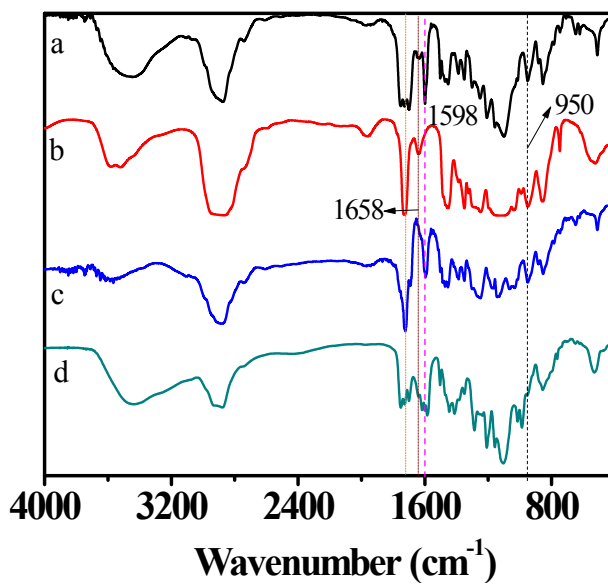
Fig. S2. FTIR spectra of (a) \text{PPEGMA}_{42} , (b) \text{PPEGMA}_{42}\text{-}b\text{-PFPMA}_{122} , (c) \text{PPEGMA}_{42}\text{-}b\text{-PFPMA}_{122}\text{-(CDs)} and (d) \text{PPEGMA}_{42}\text{-}b\text{-PFPMA}_{122}\text{-(CDs)-DOX} .
