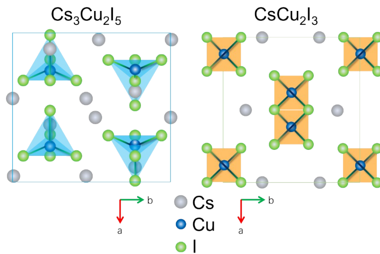
Fig. S4 Top view of the crystal structures of the \text{Cs}_3\text{Cu}_2\text{I}_5 and \text{CsCu}_2\text{I}_3 SCs.
