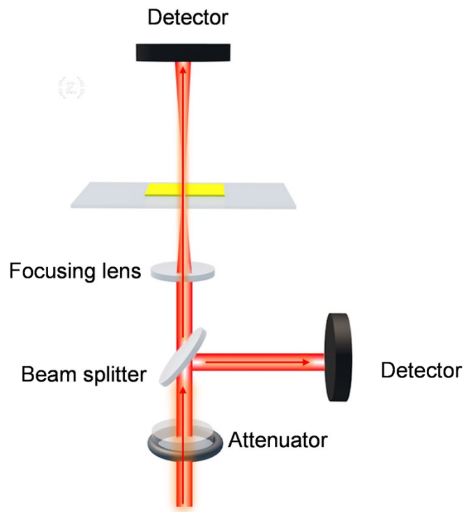
Fig. S5 The schematic diagram for our home-built micro-area nonlinear optical characterization system.
