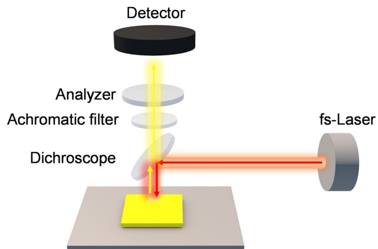
Fig. S3 The measurement configuration for two- and three-photon excited PL spectra.
