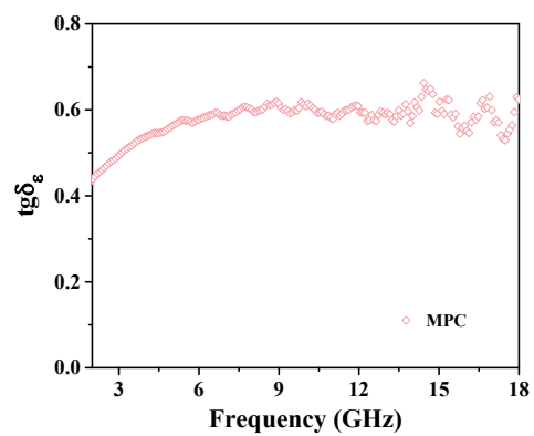
Fig. S4 The plots of \tan\delta_\epsilon versus frequency for MPC.
