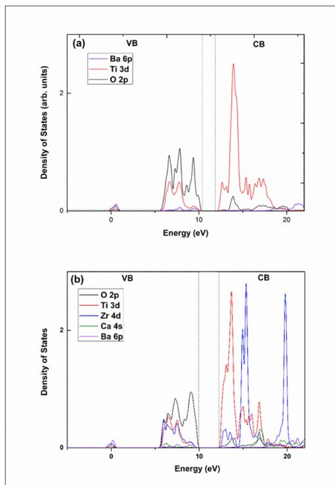
S.I. Fig. 1. Calculated partial density of states (PDOS) of BT (Tetra) and BCZT (Tetra) with constituent ions valence states.
