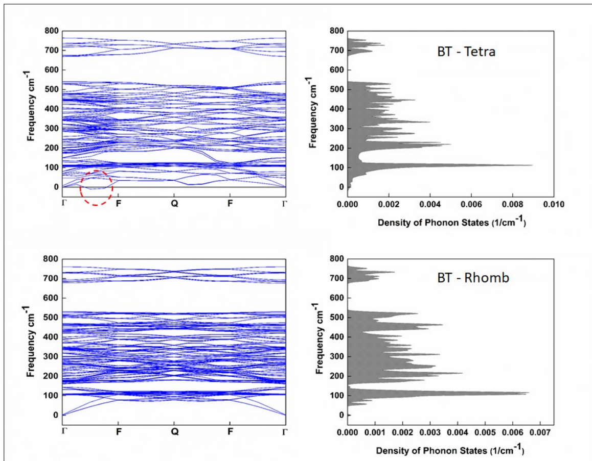
S.I. Fig. 2. Phonon dispersion and Phonon density of states of BT with tetragonal and rhombohedral structures.
