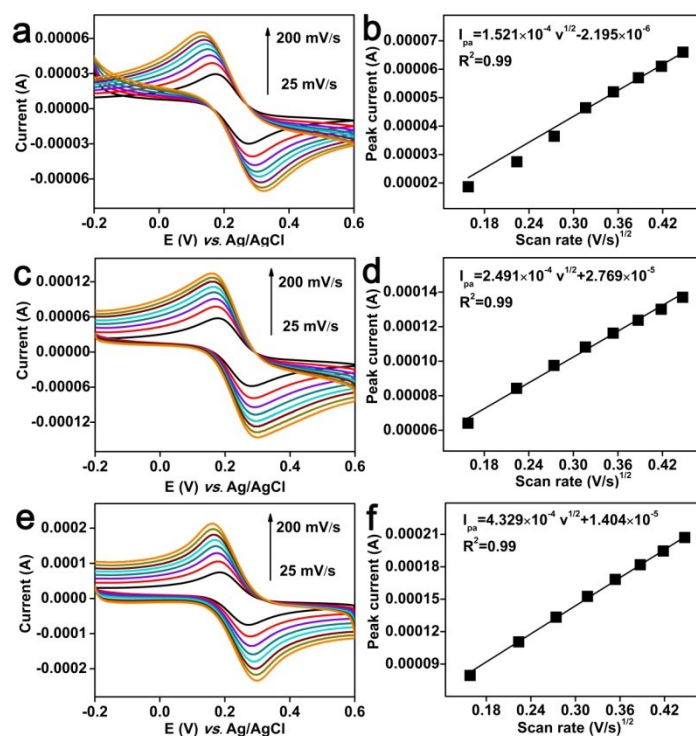
Figure S1 CV of (a) bare GCE, (c) MWCNTs/GCE, (e) ZIF-8/MWCNTs/GCE in 5 mM [Fe(CN) 6 ] 3-/4- containing 0.1 M KCl. ( v = 25, 50, 100, 125, 150, 175, and 200 mV/s). The corresponding calibration curves of (b) bare GCE, (d) MWCNTs/GCE, (f) ZIF-8/MWCNTs/GCE, respectively.
