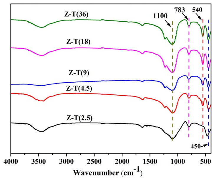
Figure S1. FTIR spectra of Z-T(2.5), Z-T(4.5), Z-T(9), Z-(18) and Z-T(36).
