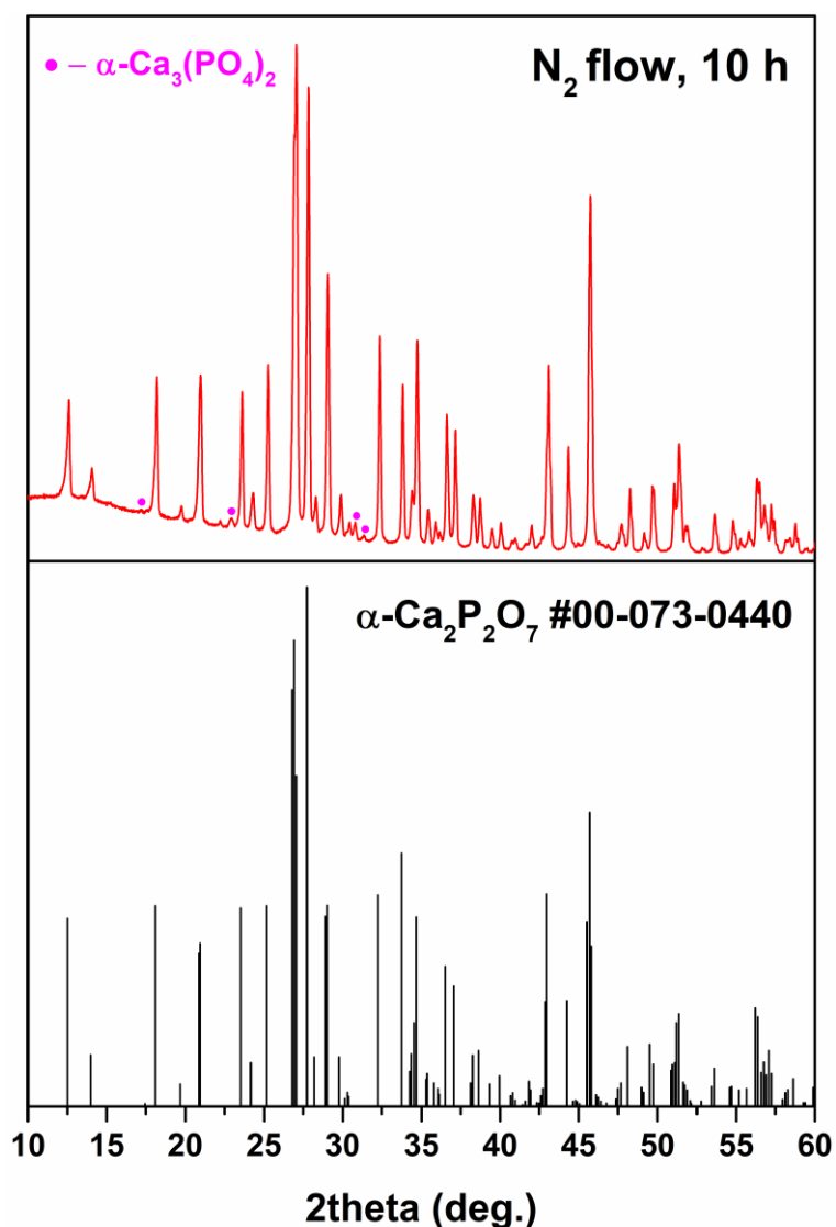
Figure S1. XRD patterns of DCPD powders annealed in N 2 flow at 1200 °C for 10 h.
