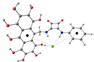
5...Cl -
