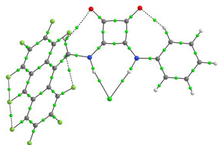
2-Cl -
