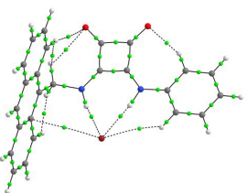
1-Br
