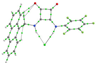
3-Cl -
