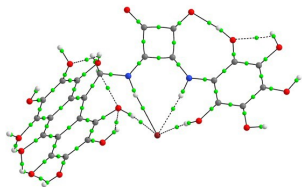
7-Br
