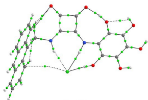
6-Cl
