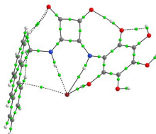
6-Br
