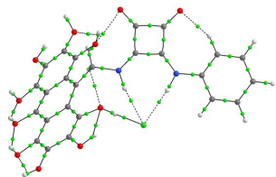
5-Cl
