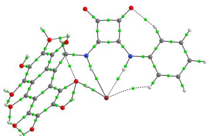
5-Br
