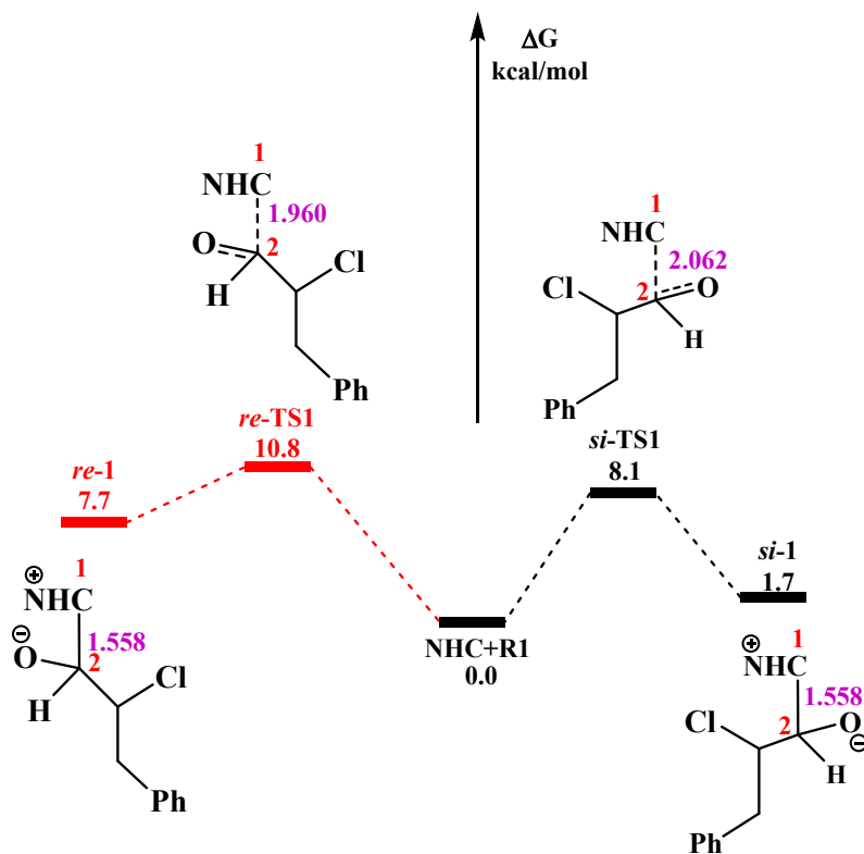
Fig. S1 Free energy surface and optimized structures for Step 1. Free energies (in kcal/mol) are at SMD(toluene)M06-2X-D3/6-311++G(2df,2pd) level. Bond lengths are given in Å.
