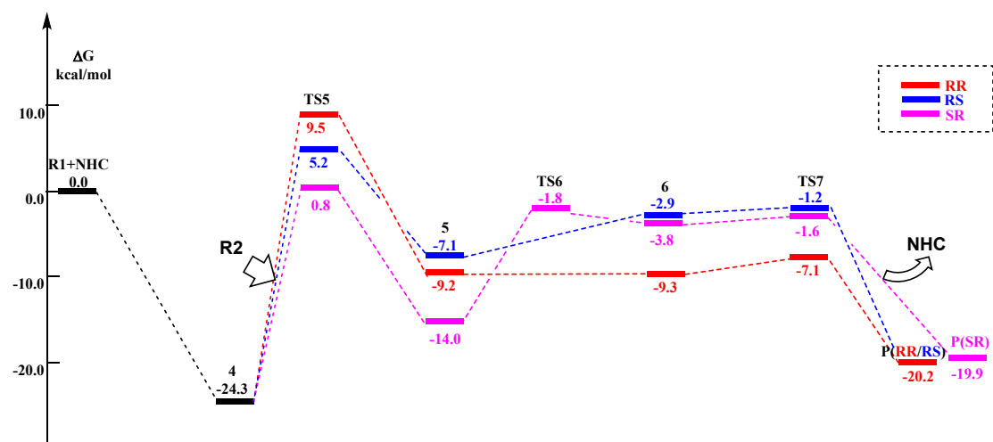
Fig. S4 Free energy surface for the unfavored pathways. Free energies (in kcal/mol) are at SMD(toluene)M06-2X-D3/6-311++G(2df,2pd) level.
