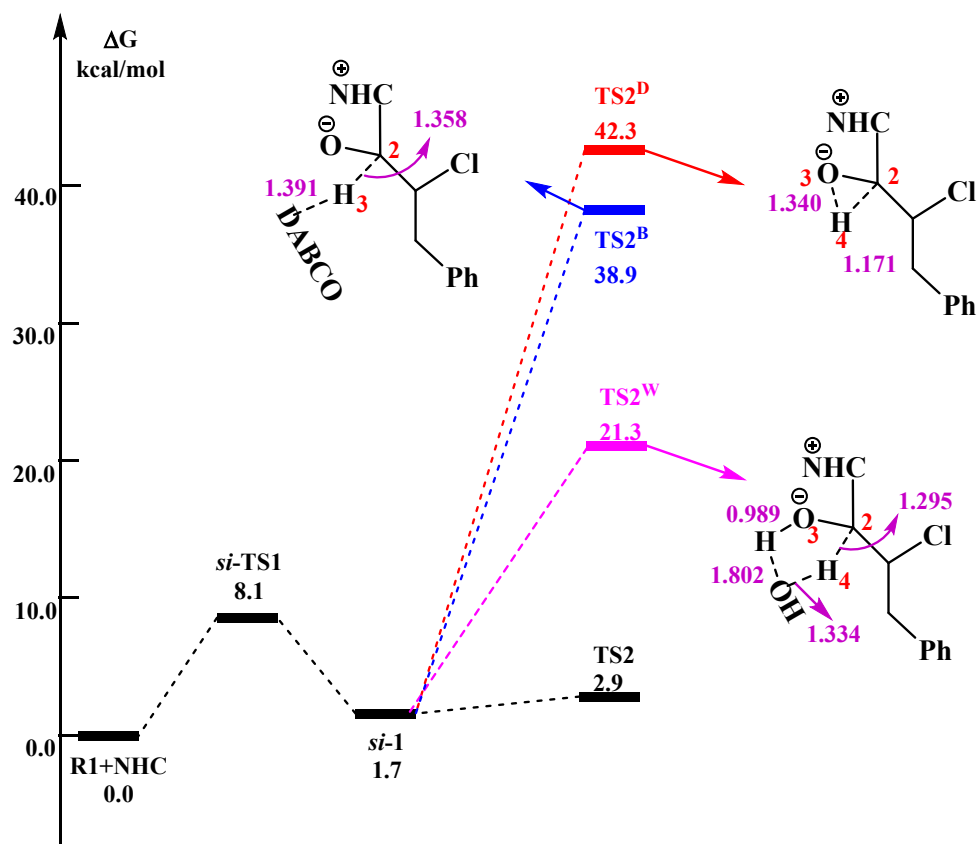
Fig. S2 Free energy surface and optimized transition states for Step 2. Free energies (in kcal/mol) are at SMD(toluene)M06-2X-D3/6-311++G(2df,2pd) level. Bond lengths are given in Å.
