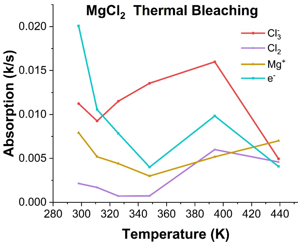
Figure S1. Thermal bleaching curves for the main transients in MgCl 2 irradiated at 100 kGy absorbed gamma dose. Cl 2 - could not be determined by overlapping with the band at 378 nm of Mg + .
