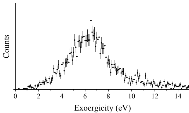
Figure SI 1: Total exoergicity spectrum for the DSET reaction, \text{Ar}^{2+} + \text{N}_2 \rightarrow \text{Ar}^+ + \text{N}^+ + \text{N} . The error bars represent two standard deviations of the associated counts.
