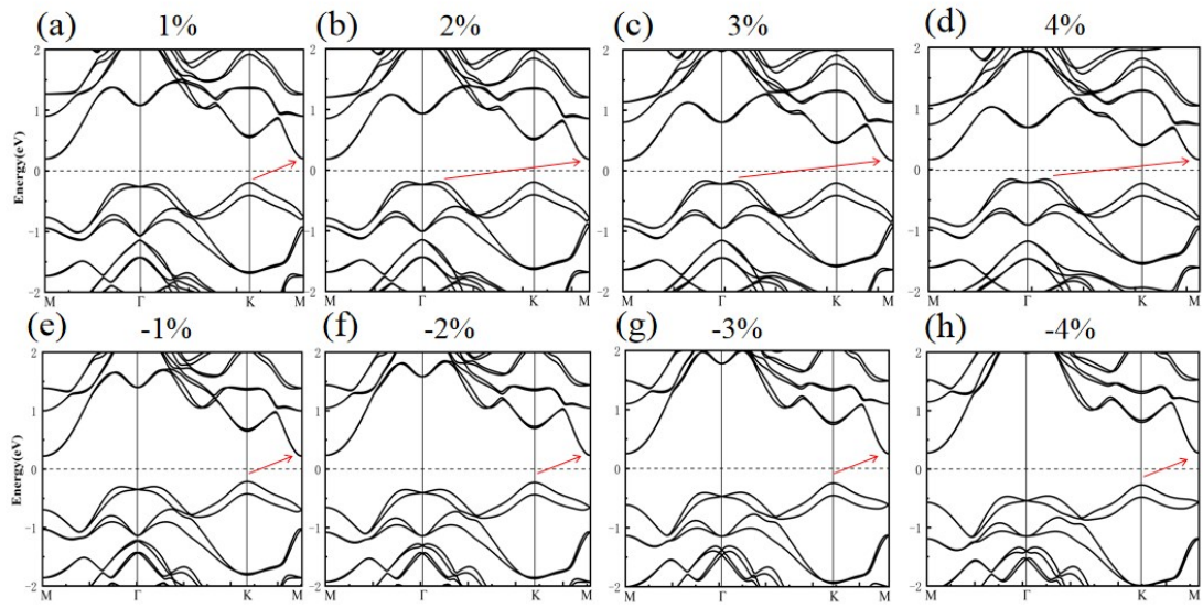
Fig S2. (a)-(h) Band structures of the 1T-SnS 2 /MoTe 2 heterostructure with biaxial strain.
