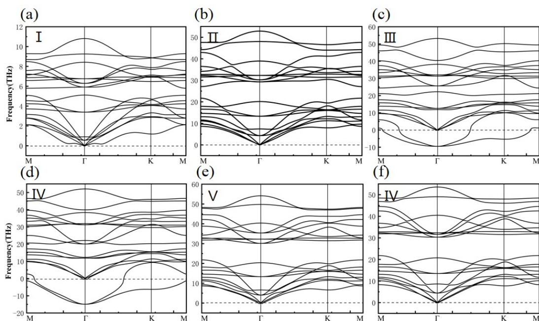
Fig S1. (a)-(f) Calculated phonon spectra for the six possible stacking configurations.
