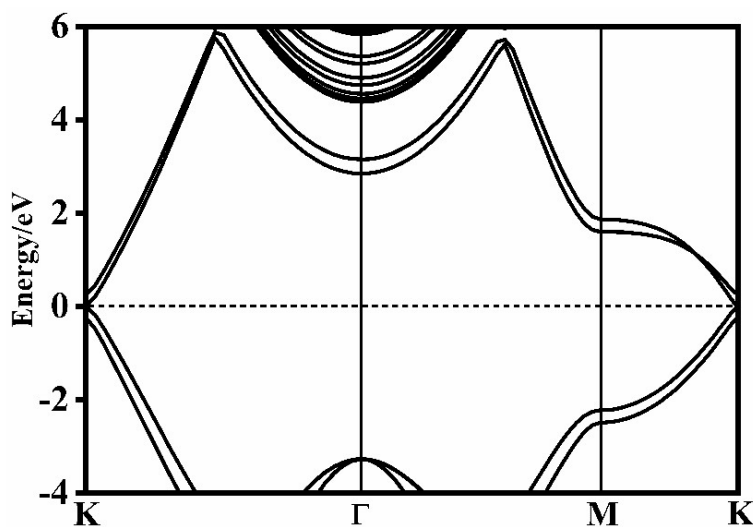
Fig. S2 Band structure of bilayer graphene with AB-stacked configuration at the PBE level.
