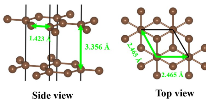
Fig. S1 Optimized structure of bilayer graphene with AB-stacked configuration.
