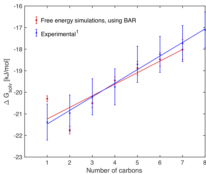
Figure S1: Free energy of solvation calculated from simulations (this study) and compared to experimental values from 1 Marenich, Aleksandr V et al Minnesota Solvation Database (MNSOL) version 2020
