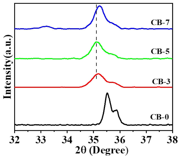
Figure S2. Powder X- ray diffraction peak shift
