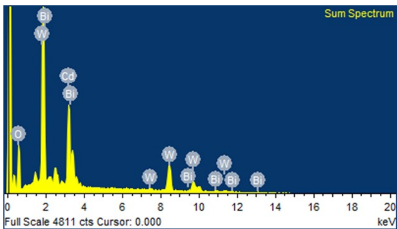
Figure S3. EDX spectra of CB-5 sample.
