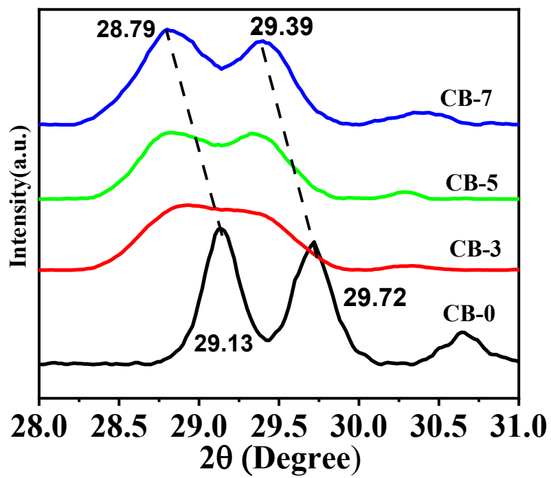
Figure S1. Powder X- ray diffraction peak shift
