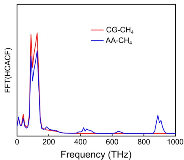
Figure S1 Fast Fourier Transform (FFT) of HCACF of monocrystalline sI clathrate hydrate (AA: blue, CG: red).
