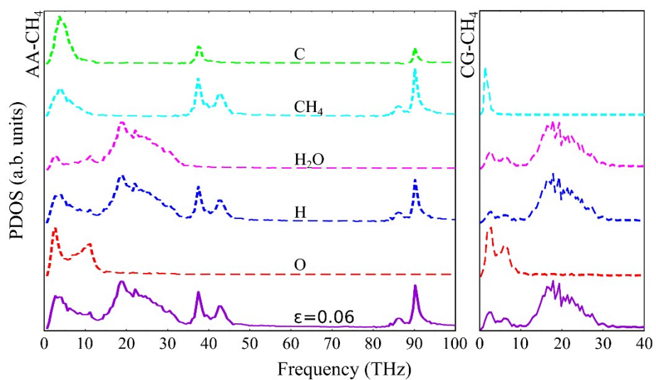
Figure S2 PDOS of sI methane hydrate with (a) AA and (b) CG models of methane molecule at triaxial tension strain of 0.06.
