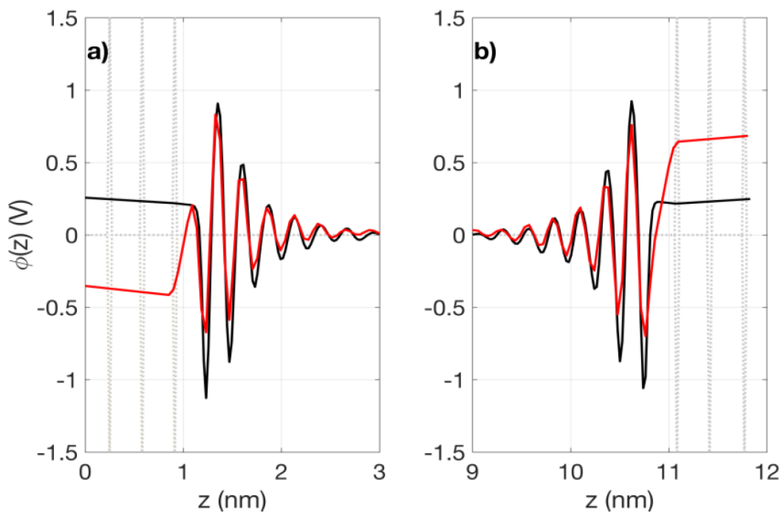
Figure S1 - Electrostatic potential profile (V), in two different applied potentials (0 and 1.2 V) for \text{Li}_2\text{SO}_4 as a function of electrodes distance, z (nm).
