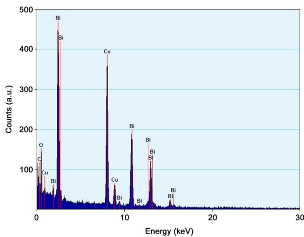
Fig. S1. EDS spectrum of 3h-BOC.
