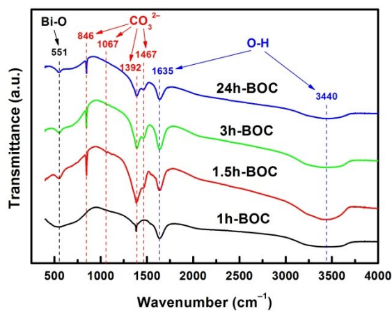
Fig. S2. FTIR spectra of BOC samples derived at different reaction times.
