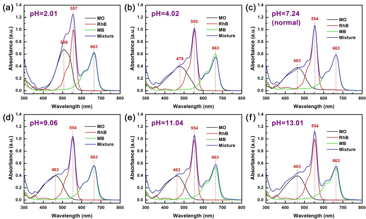
Fig. S3. UV-vis absorption spectra of fresh MO, RhB, MB, and MO/RhB/MB mixture solutions at different pH values.
