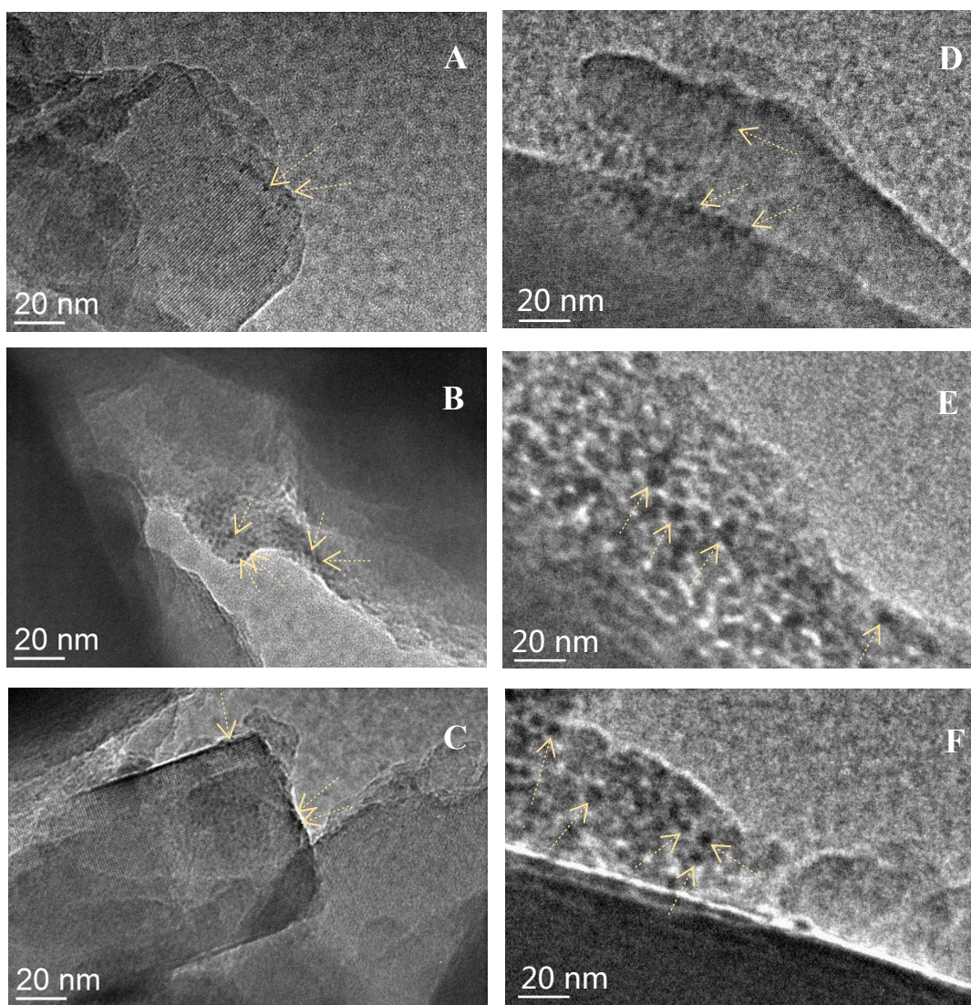
Fig. S1. The TEM images of the PtZn/0.02TS-95 (A, B, C) and PtZn/S-95 (D, E, F).
