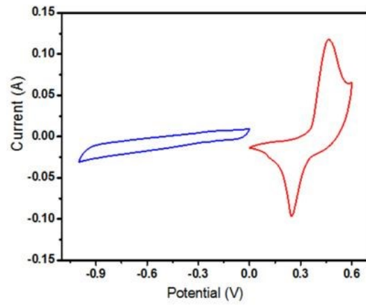
Fig. S5 CV curves of the AC and C-NMO@MX electrode, which were recorded at 4 mV s -1 .
