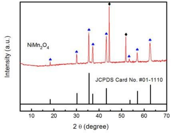
Fig. S3 XRD patterns of the NiMn 2 O 4 nanosheets.
