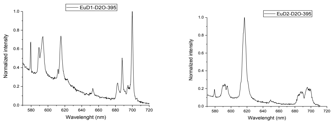
Fig. S21 Luminescence spectra of [\text{Eu}(\text{L}_1)]^{3+} (left) and [\text{Eu}(\text{L}_2)]^{3+} (right) in \text{D}_2\text{O}
