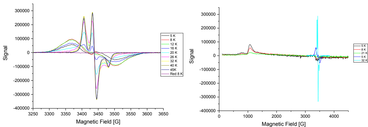
Fig. S5 Low temperature evolution of the EPR spectrum of a 0.45 mM aqueous solution (containing 10% glycerol) of [\text{Yb}(\text{L}_1)]^{3+} . Microwave Freq; 9.63 GHz, power 0.2 mW; Mod. Freq. 100 KHz, Amp. 0.4 mT.
