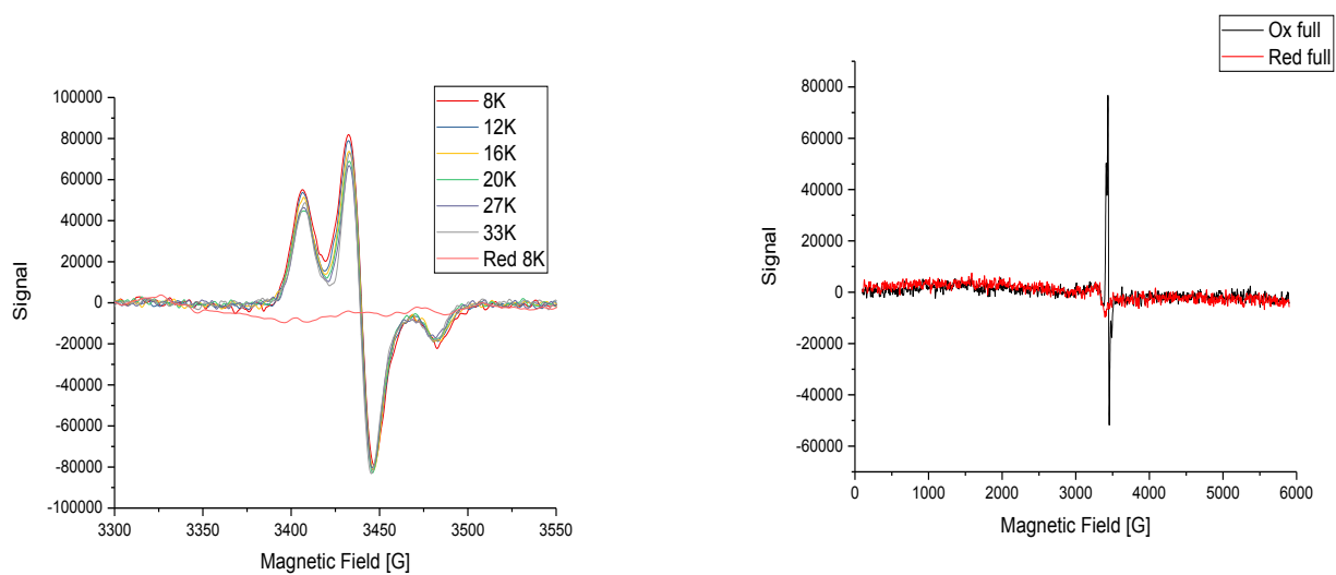
Fig. S7 Low temperature evolution of the EPR spectrum of a 0.45 mM aqueous solution (containing 10% glycerol) of [\text{Eu}(\text{L}_1)]^{3+} . Microwave Freq; 9.63 GHz, power 0.2 mW; Mod. Freq. 100 KHz, Amp. 0.4 mT.
