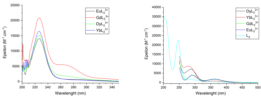
Fig. S2 UV-Vis spectra of 0.5 mM solution of \text{YbL}_2^{3+} , \text{DyL}_2^{3+} , \text{EuL}_2^{3+} and \text{GdL}_2^{3+} (Left : in Water, Right : in MeCN)
