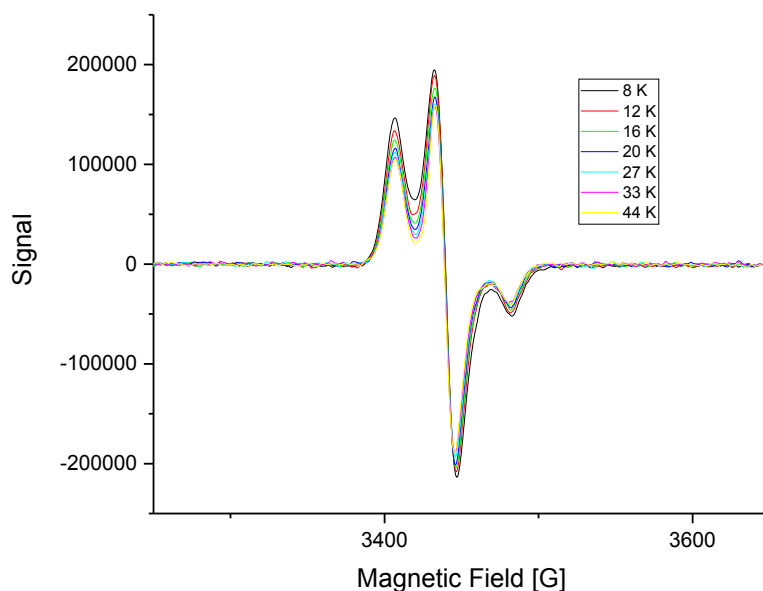
Fig. S10 Low temperature evolution of the EPR spectrum of a 0.45 mM aqueous solution (containing 10% glycerol) of [\text{Eu}(\text{L}_2)]^{3+} . Microwave Freq; 9.63 GHz, power 0.2 mW; Mod. Freq. 100 KHz, Amp. 0.4 mT.
