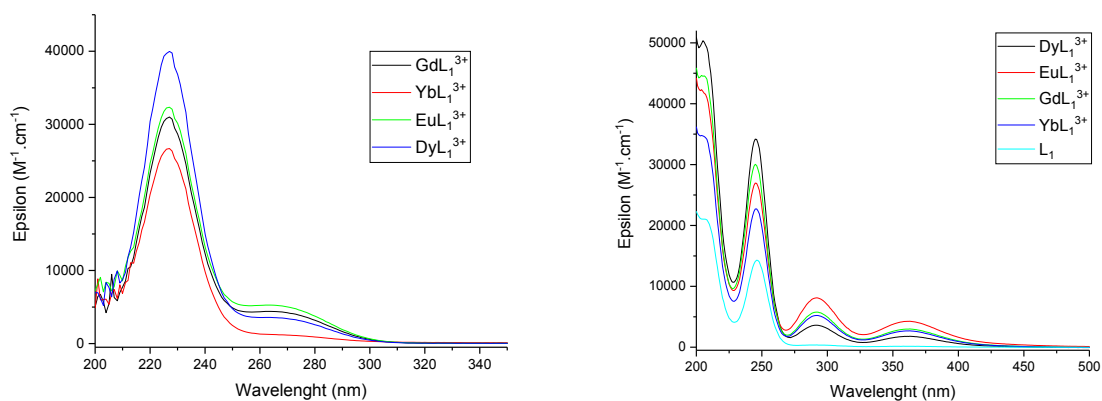
Fig. S1 UV-Vis spectra of 0.5 mM solution of \text{YbL}_1^{3+} , \text{DyL}_1^{3+} , \text{EuL}_1^{3+} and \text{GdL}_1^{3+} (Left : in Water, Right : in MeCN)
