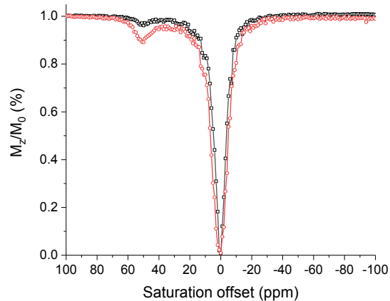
Fig. S18 CEST spectra of 14 mM solution of [\text{Eu}(\text{L}_1)]^{3+} in oxidized (black) and reduced (red) forms using sodium ascorbate. Recorded at 11.7 T, 298 K, in mixture of 0.1M HEPES buffer pH 7.4 and \text{CD}_3\text{CN} (2/1), B_1 = 25 \mu\text{T} , and irradiation time of 3 s.
