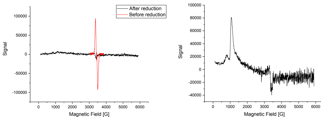
Fig. S13 X-Band EPR spectrum of [\text{Yb}(\text{L}_1)]^{3+} after addition of 2 molar equiv. of ascorbate. Microwave Freq; 9.63 GHz, power 0.2 mW (left), 2 mW (right); Mod. Freq. 100 KHz, Amp. 0.4 mT (left), 1 mT (right). T = 7K (left), 5K (right).
