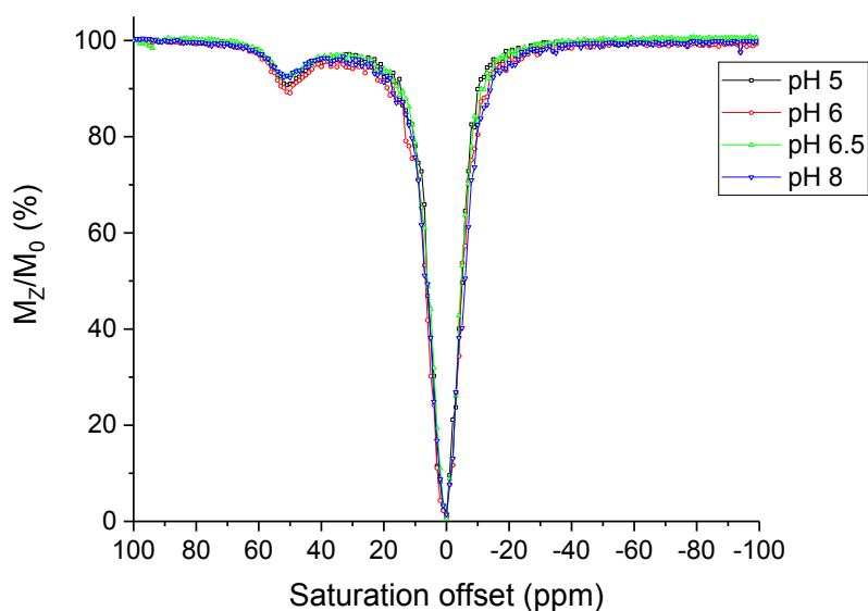
Fig. S16 PARACEST spectra of [\text{Eu}(\text{L}_1)]^{3+} as a function of the pH. CEST at +51 ppm coming from the coordinated water molecules of the hydroxylamine \text{Eu}^{3+} complexes recorded at 11.7 T, 298 K, B_1 = 1064 Hz (25 \mu\text{T} ), concentration = 12 mM (66% \text{H}_2\text{O} -HEPES buffer 0.1M in \text{CD}_3\text{CN} ) and irradiation time = 3 s.
