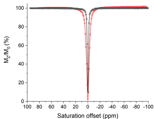
Fig. S20 CEST spectra of 20 mM solution of [\text{Eu}(\text{L}_2)]^{3+} in oxidized (black) and reduced (red) forms using 2 eq of sodium ascorbate. Recorded at 11.7 T, 298 K, in mixture of 0.1M HEPES buffer pH 7.4 and \text{CD}_3\text{CN} (2/1), B_1 = 25 \mu\text{T} , and irradiation time of 3 s.
