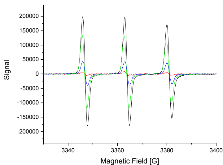
Fig. S15 X-Band EPR spectrum of a 0.5 mM solution of [\text{Gd}(\text{L}_2)]^{3+} in water with HEPES buffer at pH 7. (black) initial; (red) after addition of 1 molar equivalent of ascorbate; (green) after addition of 1 molar equivalent of ascorbate followed by addition of \text{NaIO}_4 in excess and 30 min reaction; (blue) after addition of 1 molar equivalent of ascorbate followed by increase of pH to 13 and dioxygen bubbling during 30 min. Microwave Freq; 9.42 GHz, power 3.5 mW; Mod. Freq. 100 KHz, Amp. 0.2 mT. T = 293 K.
