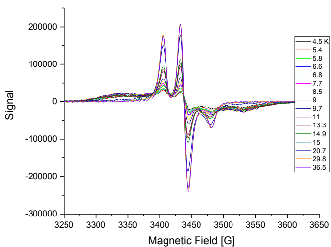
Fig. S8 Low temperature evolution of the EPR spectrum of a 0.45 mM aqueous solution (containing 10% glycerol) of [\text{Yb}(\text{L}_2)]^{3+} . Microwave Freq; 9.63 GHz, power 2 mW; Mod. Freq. 100 KHz, Amp. 0.4 mT.
