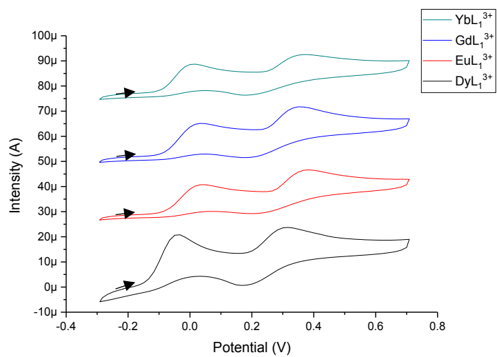
Fig. S3 CV curves of 0.5 mM solution of \text{YbL}_1^{3+} , \text{DyL}_1^{3+} , \text{EuL}_1^{3+} and \text{GdL}_1^{3+} in \text{CH}_3\text{CN} containing TBAP. Scan rate = 0.1 V/sec; Ref:Fc + /Fc.
