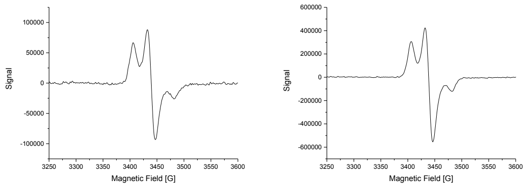
Fig. S11 X-Band EPR spectra of 0.45 mM aqueous solutions (containing 10% glycerol) of L_1 (left) and L_2 (right). Microwave Freq; 9.63 GHz, power 2 mW; Mod. Freq. 100 KHz, Amp. 0.4 mT. T = 8.8 K (left), 10.7 K (right).
