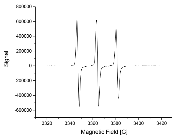
Fig. S12 X-Band EPR spectrum of a 0.5 mM solution of L_2 in water with HEPES buffer at pH 7.9. Microwave Freq; 9.42 GHz, power 3.5 mW; Mod. Freq. 100 KHz, Amp. 0.2 mT. T = 293 K.
