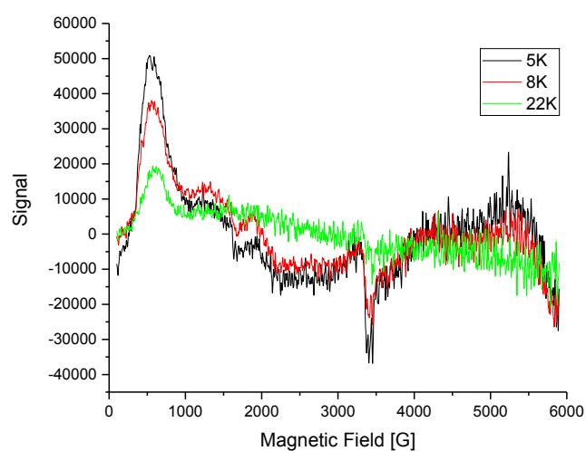
Fig. S14 Low temperature evolution of the X-Band EPR spectrum of [\text{Dy}(\text{L}_1)]^{3+} after addition of 2 molar equiv. of ascorbate. Microwave Freq; 9.63 GHz, power 2 mW; Mod. Freq. 100 KHz, Amp. 1 mT.
