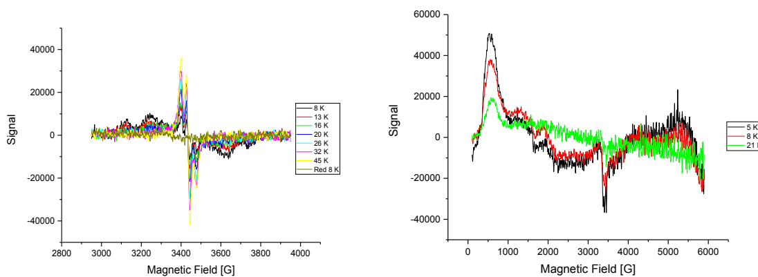
Fig. S6 Low temperature evolution of the EPR spectrum of a 0.45 mM aqueous solution (containing 10% glycerol) of [\text{Dy}(\text{L}_1)]^{3+} . Microwave Freq; 9.63 GHz, power 4 mW; Mod. Freq. 100 KHz, Amp. 0.4 mT.
