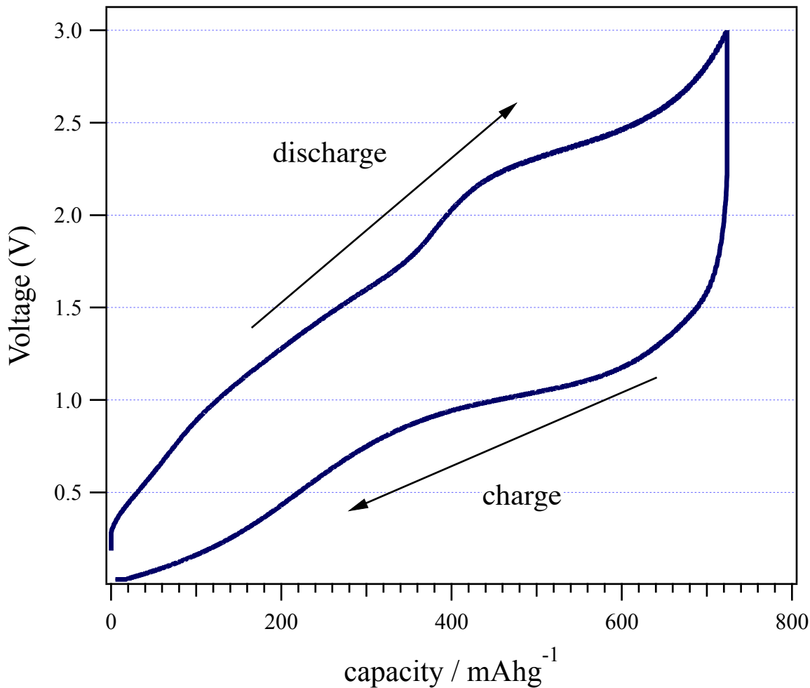
Fig. S1. Charge-discharge curve of NiO in the third cycle.
