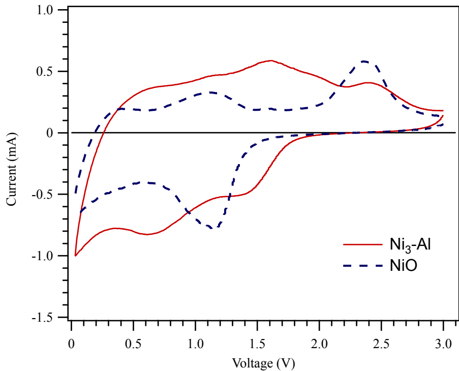
Fig. S2. Cyclic voltammograms of NiO and Ni 3 AlO recorded at a scan rate of 0.1 \text{ mV s}^{-1} .
