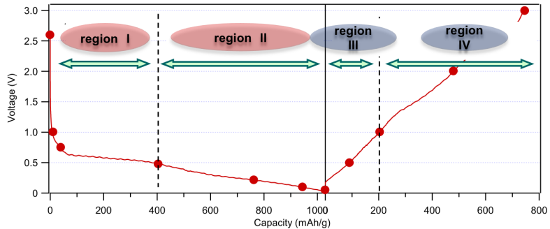
Fig. S4. The charge-discharge curves of Ni 2 AlO in the first cycle.
