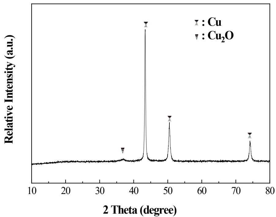
Figure S3. XRD pattern of Cu-t-6
