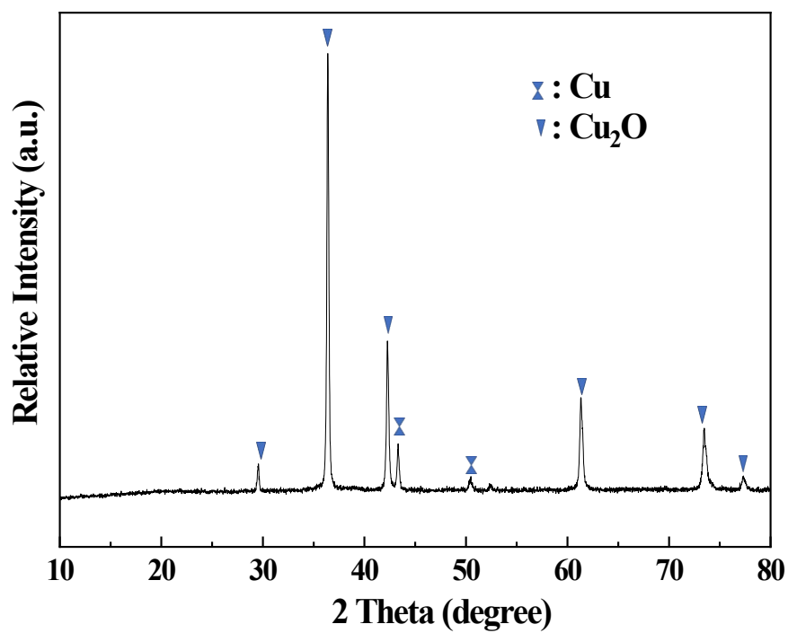
Figure S2. XRD pattern of Cu-t-3
