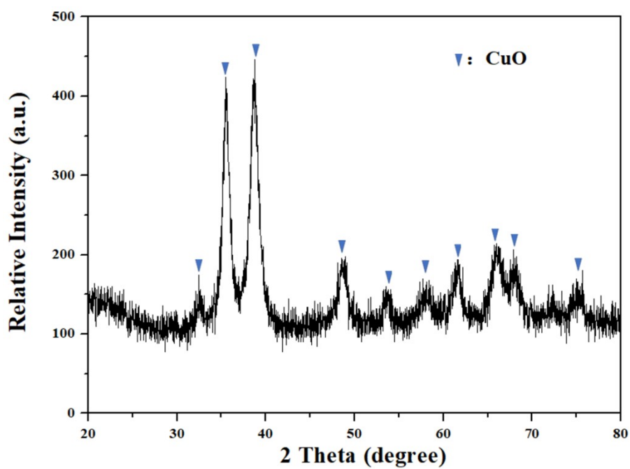
Figure S1. XRD pattern of Cu-t-0
