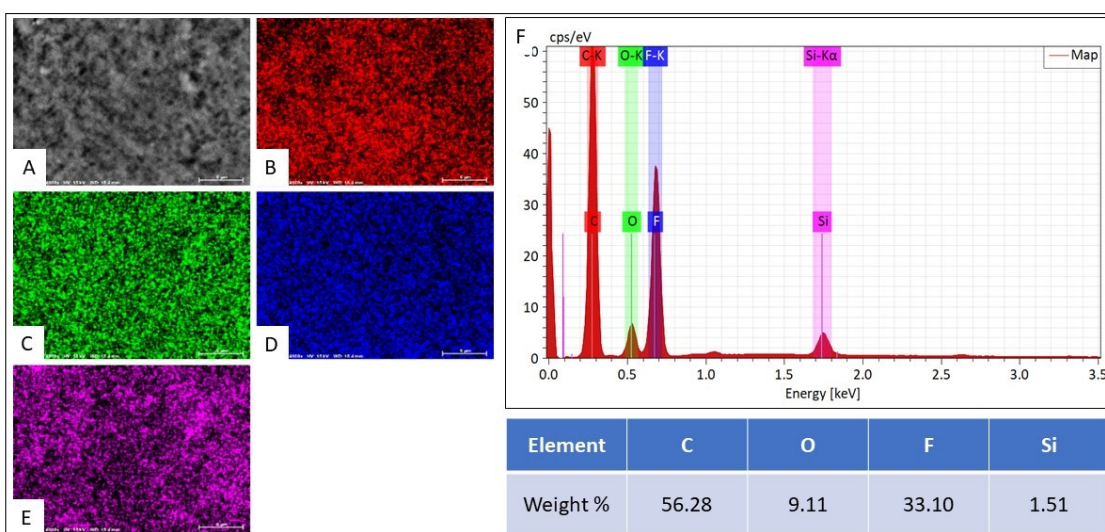
Figure S2 EDX Results of AS Membrane. A. SEM image; B. Carbon(C) Element Mapping; C. Oxygen(O) Element Mapping; D. Fluoride(F) Element Mapping; E. Silicon(Si) Element Mapping; F. EDX Spectrum.
