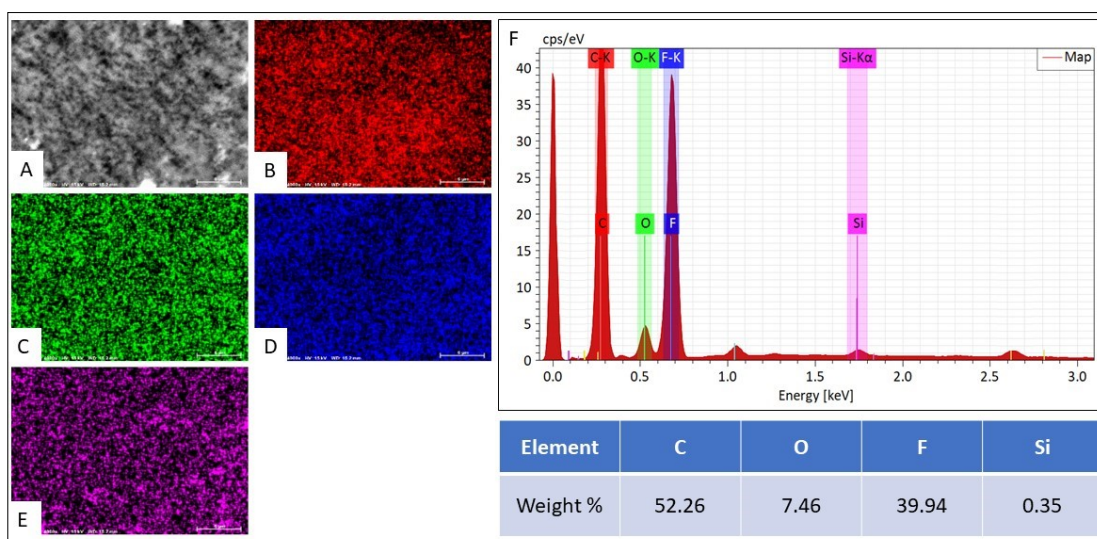
Figure S1 EDX Results of MS Membrane. A. SEM image; B. Carbon(C) Element Mapping; C. Oxygen(O) Element Mapping; D. Fluoride(F) Element Mapping; E. Silicon(Si) Element Mapping; F. EDX Spectrum.
