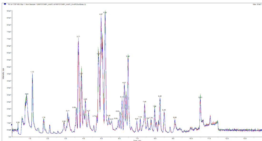
Figure S2: Overlaid chromatogram of QC injection in positive ion mode (A) and negative ion mode (B).
