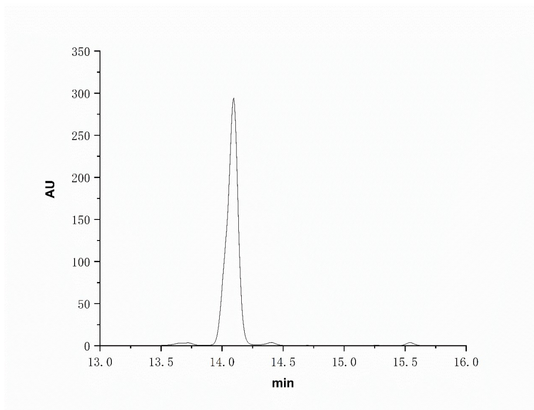
High-performance liquid chromatography (HPLC) chromatograms of Mv3C
