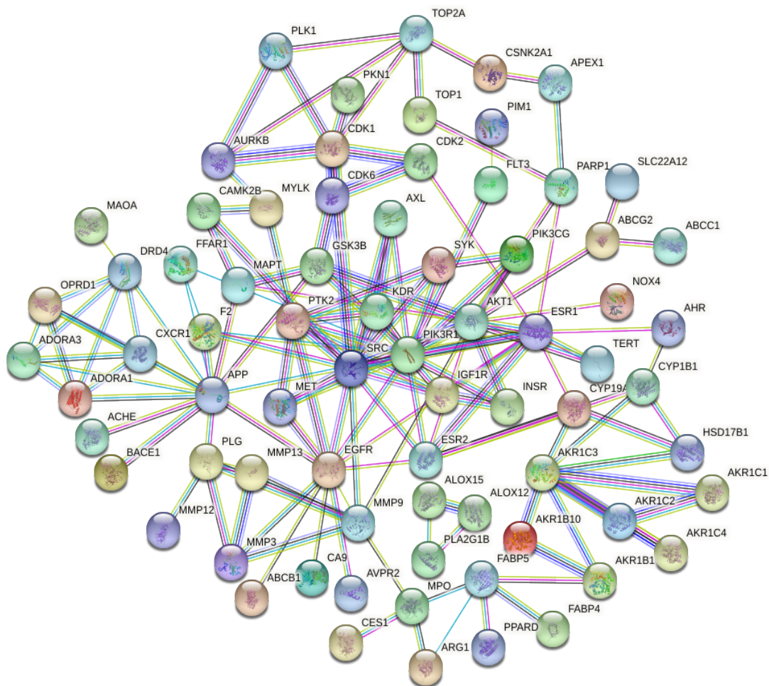
Figure S1: The core hub of PPI network
