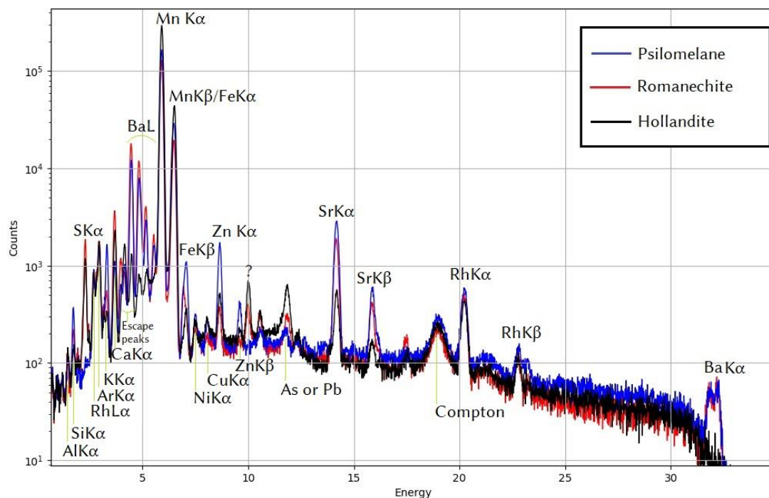
Figure 2: Spectra of the psilomelane, romanechite and hollandite raw materials used to prepare the mock-ups.
