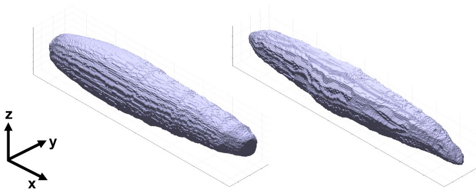
Fig. S6 Reconstruction model of rotated E. gracilis .
