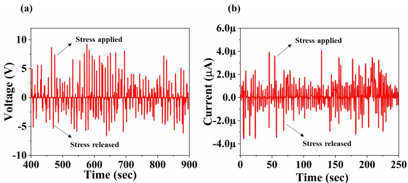
Fig. S1: The piezoelectric output of BTMO nanosheets, (a) Output voltage, (b) Output current.
