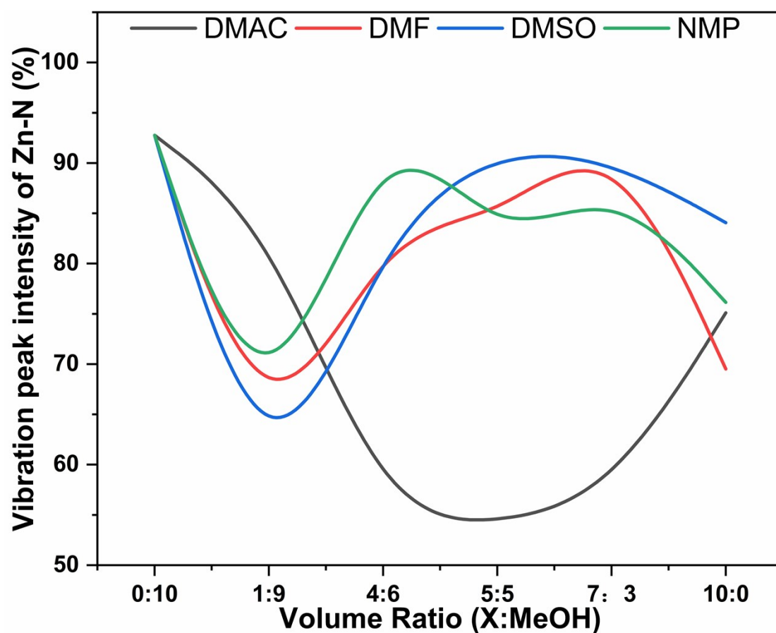
Fig. S1 Volume ratio of the binary solvent system versus vibration peak intensity of Zn-N (near 420 cm -1 )
