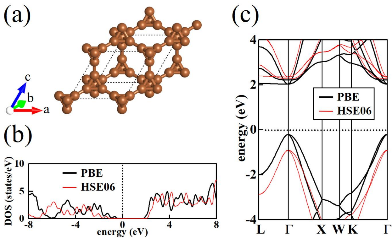
Fig. S2 The structure (a), DOS (b) and energy bands (c) of T-carbon.
