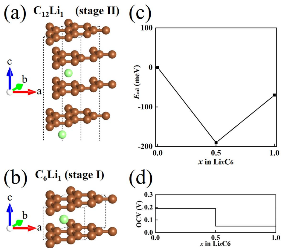
Fig. S1 The structures of graphite with Li intercalation: (a) C_{12}Li_1 and (b) C_6Li_1 . (c) The Li adsorption energy on C_{12}Li_1 and C_6Li_1 . (d) The calculated potential of graphite anode at the level of PBE-D3.
