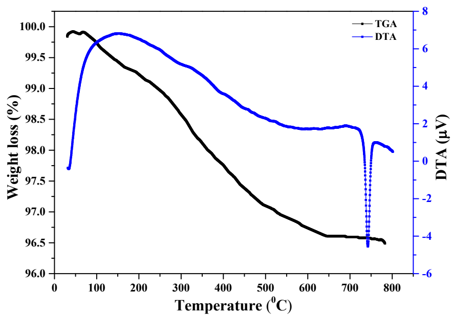
Fig. S2: TGA/DTA curves of GDBC nanocomposite solid electrolyte with 40 wt. % of CeO 2 .
