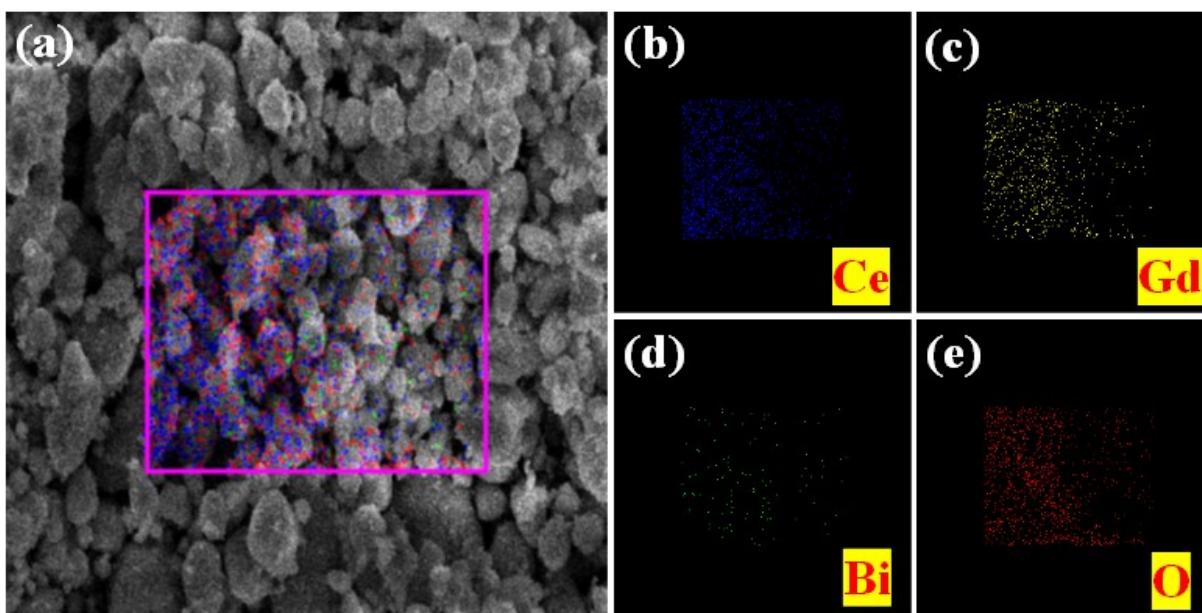
Fig. S1: Elemental mapping of Ce, Gd, Bi, and O of GDBC nanocomposite solid electrolyte with 40 wt. % CeO 2 .
