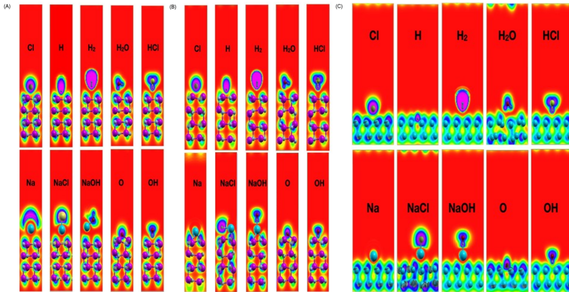
Figure S1: Electron localization function of the complex systems comprising of the molecules and ions adsorbed on different surfaces with VdW forces (A) on AlN surface (B) GaN surface (C) Si surface.
