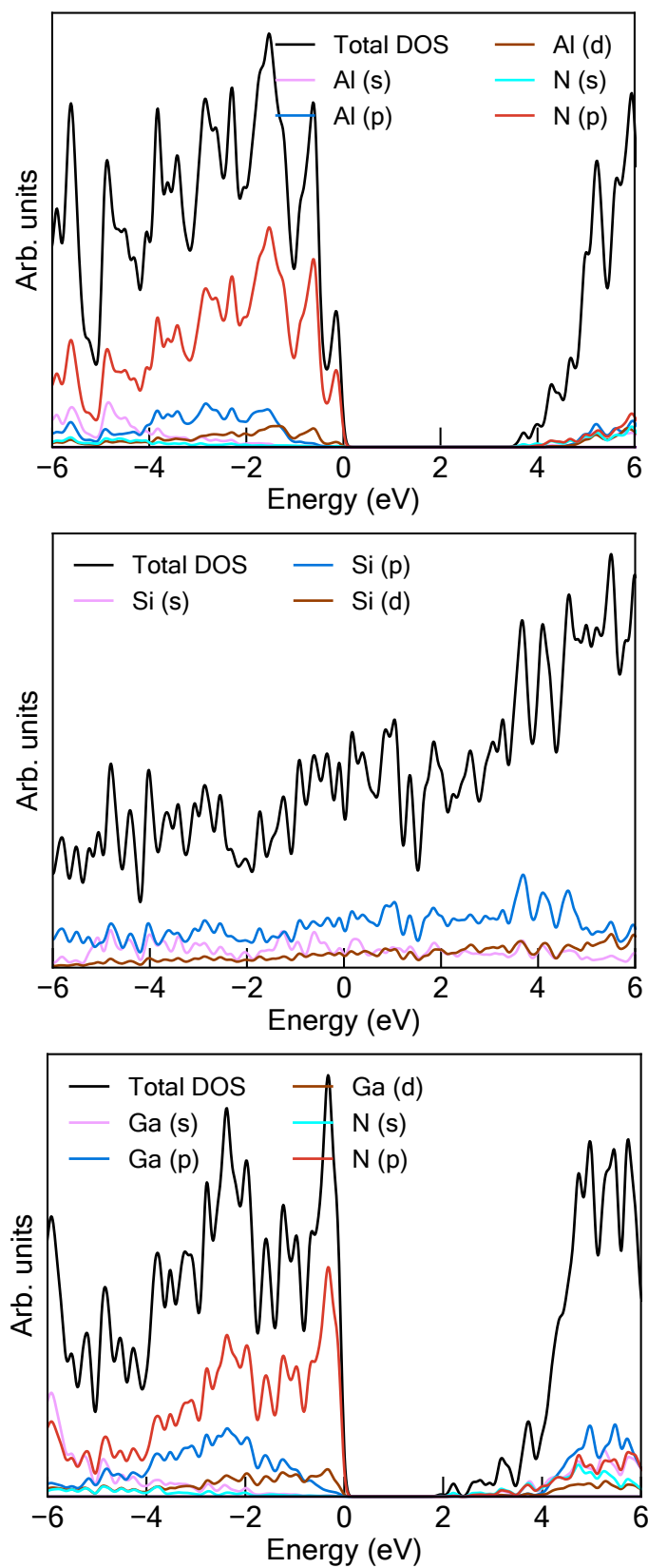
Figure S3: Projected Density of States of the pristine surfaces without VdW forces.
