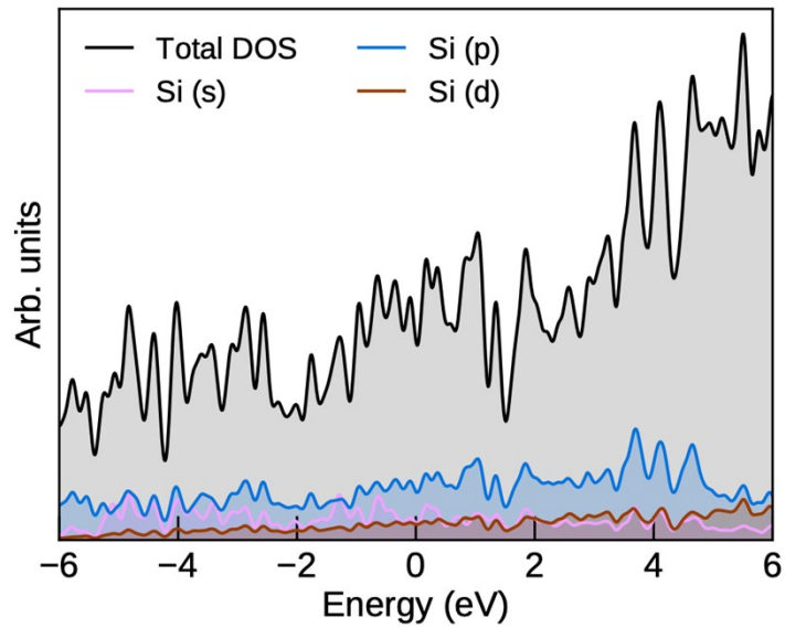
Figure S2: Projected Density of States of the pristine surfaces with VdW forces.
