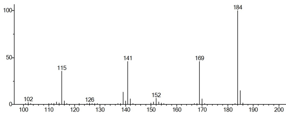
Fig. S3. GC-MS spectrum of p-methoxy-biphenyl (Entry 1 and 5 in Table 3)
