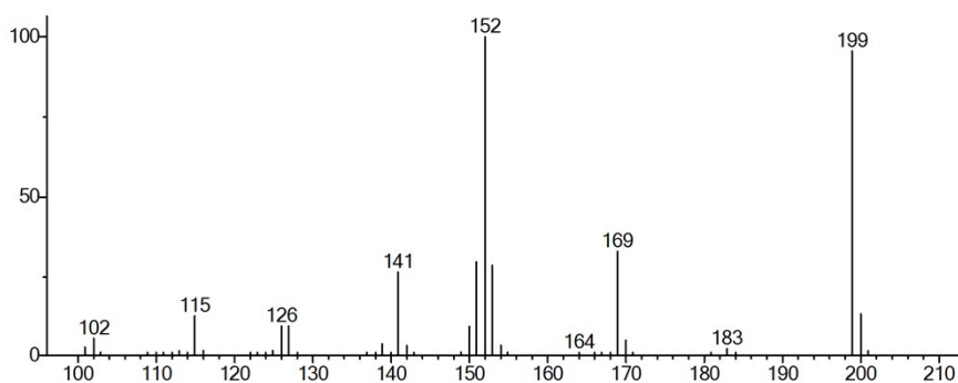
Fig. S4. GC-MS spectrum of p-nitro biphenyl (Entry 2 and 6 in Table 3)
