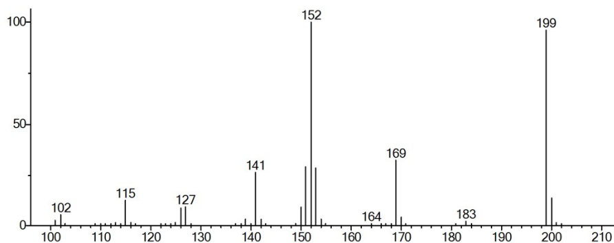
Fig. S5. GC-MS spectrum of m-nitro biphenyl (Entry 3 and 8 in Table 3)
