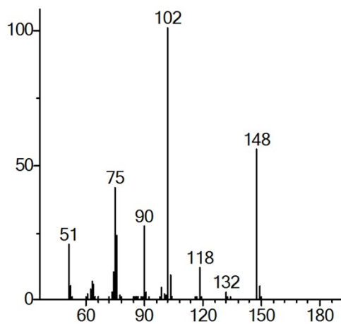
Fig. S9. GC-MS spectrum of p-nitrobenzotrile (Entry 2 and 6 in Table 6)
