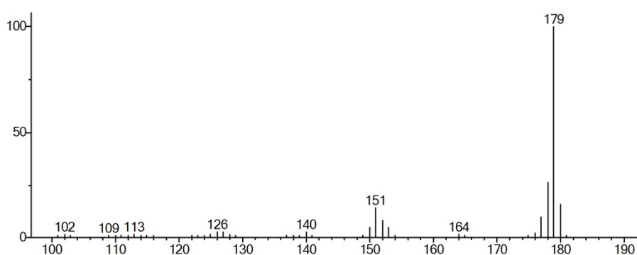
Fig. S7. GC-MS spectrum of p-cyanobiphenyl (Entry 8 in Table 3)
