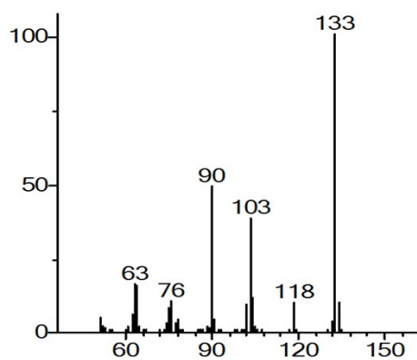
Fig. S8. GC-MS spectrum of p-methoxybenzotrile (Entry 1 and 5 in Table 5)
