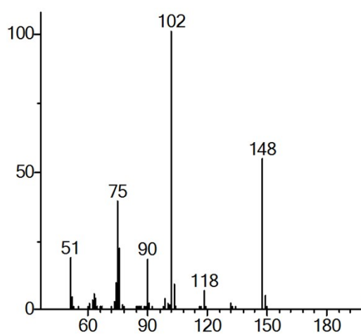
Fig. S10. GC-MS spectrum of m-nitrobenzotrile (Entry 3 and 8 in Table 6)
