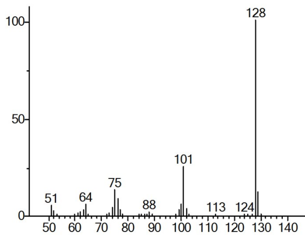
Fig. S12. GC-MS spectrum of terephthalonitrile (Entry 7 in Table 5)
