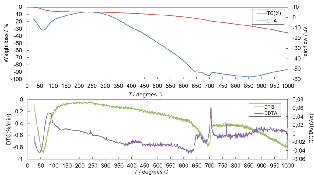
Figure S1. Thermogravimetric and differential thermal analysis of PTB
