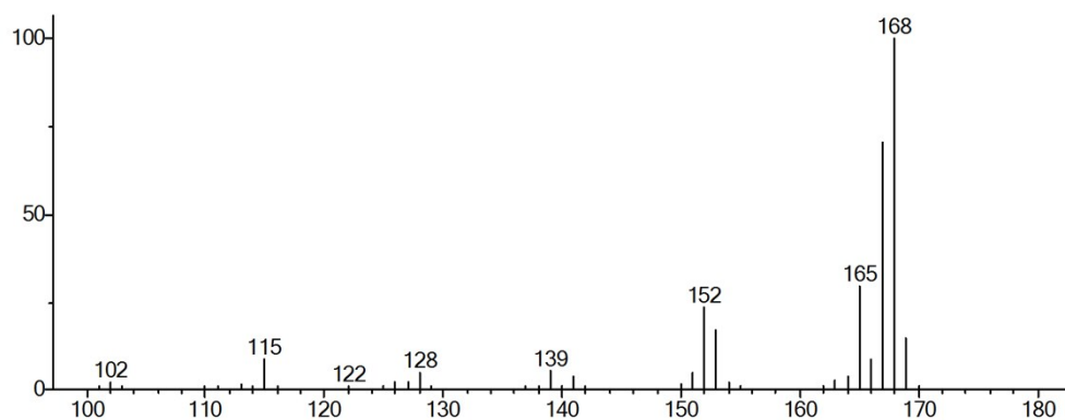
Fig. S6. GC-MS spectrum of p-methyl biphenyl (Entry 4 and 9 in Table 3)
