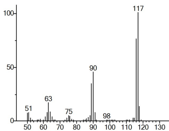
Fig. S11. GC-MS spectrum of p-tolunitrile (Entry 4 and 9 in Table 5)
