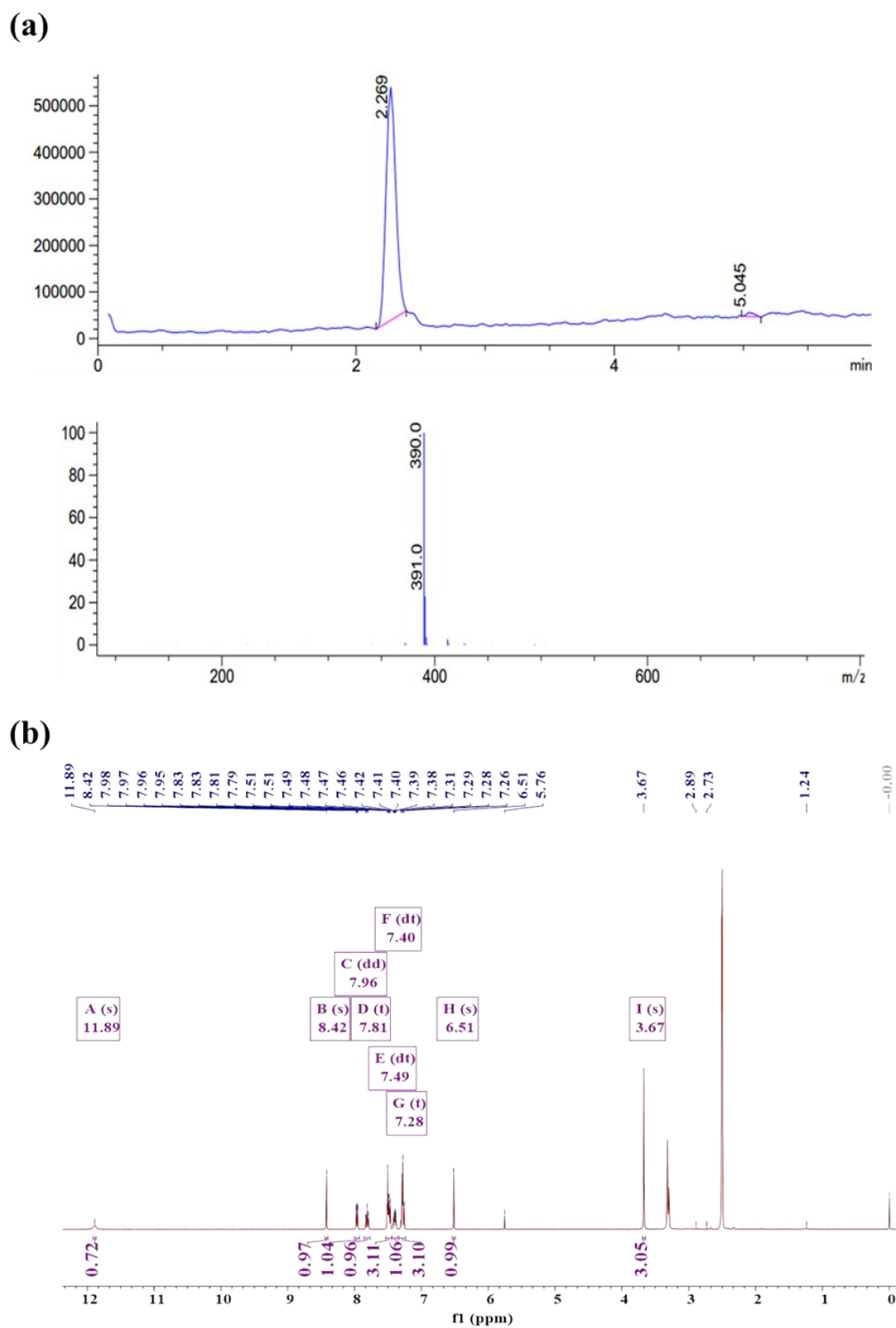
Fig. S1. (a) The LC-MS results of AZX hapten; (b) ^1\text{H} NMR results of AZX hapten.
