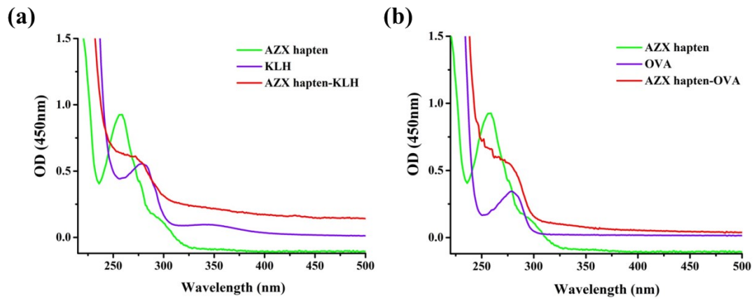
Fig. S2. UV spectrum of AZX hapten, KLH, OVA, AZX hapten-KLH, and AZX hapten-OVA: (a) immunogen; (b) coating antigen.
