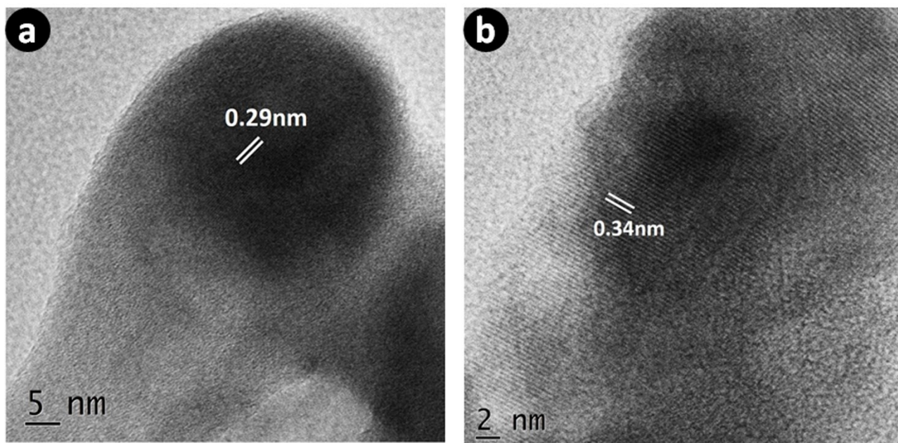
Figure S2: HR-TEM images of LMN6 (a and b)
