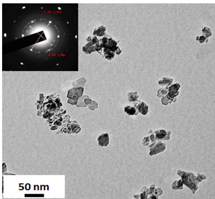
Figure S1: TEM microstructure of MN (SEAD pattern in the inset)
