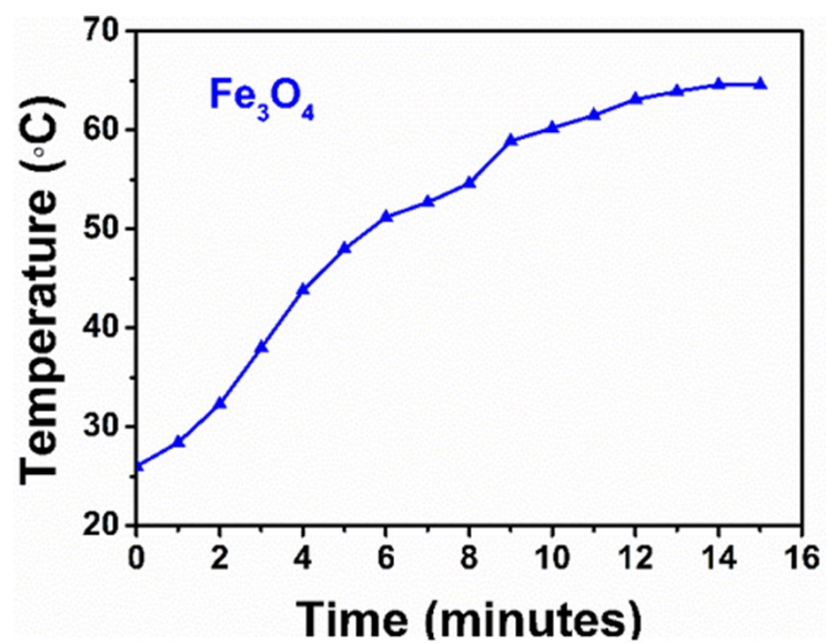
Figure S4: Time-temperature heating profile of \text{Fe}_3\text{O}_4
