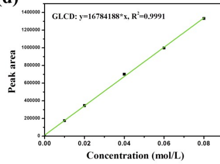
Fig. S1 Standard curves of glycerol and oxidation products
