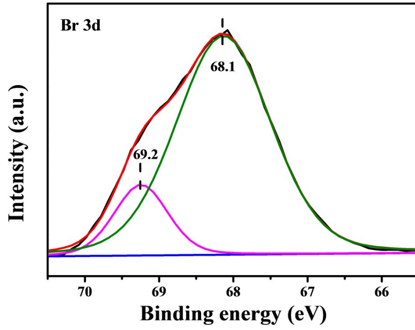
Fig. S2 XPS spectrum of Br in Bi QDs /BiOBr-O v
