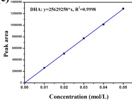
Fig. S1 Standard curves of glycerol and oxidation products
