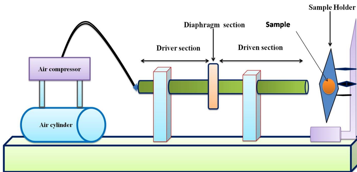
Fig.1 Schematic diagram of the shock wave loading setup
