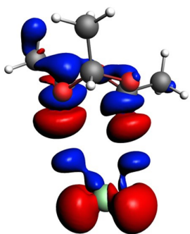
2...Cl -e
