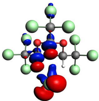
5...Cl -*
