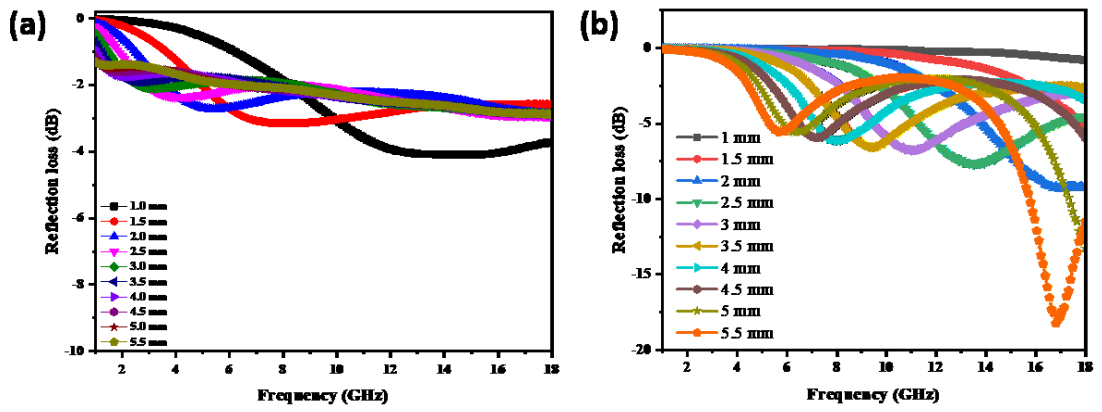
Fig. S1. The reflection loss curves dependence on the frequency and the thickness of (a) pure C and (b) the mixture of SiO 2 @C and NiCo 2 O 4 with the composition of 1:3.
