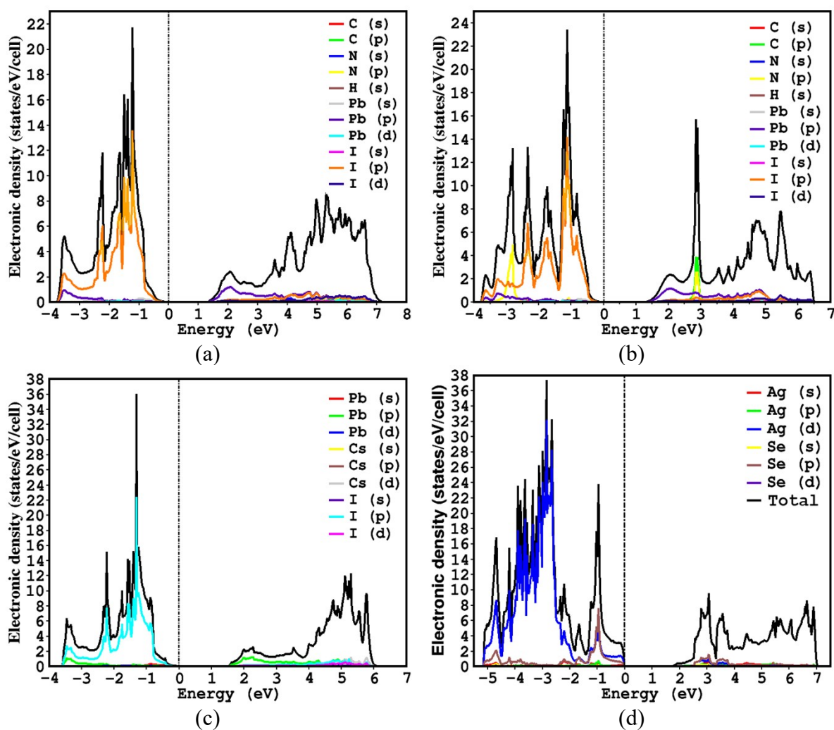
S1 Computed projected density of states (PDOS) for (a) \alpha -MAPbI 3 , (b) \alpha -FAPbI 3 , (c) \alpha -CsPbI 3 and (d) monolayer Ag 4 Se 2 phases.
