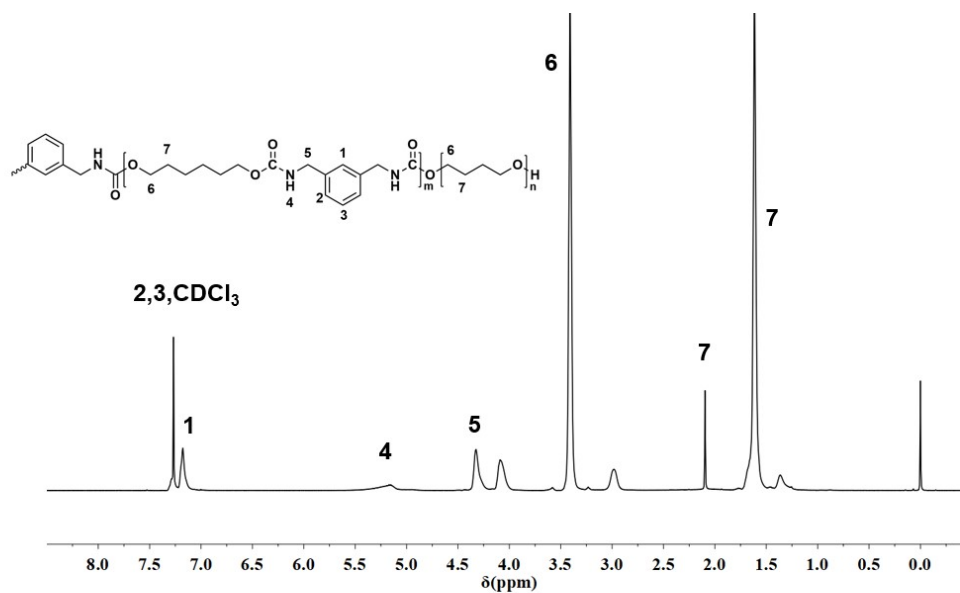
Fig. S4. 1 H NMR spectrum of XDI-PUE.
