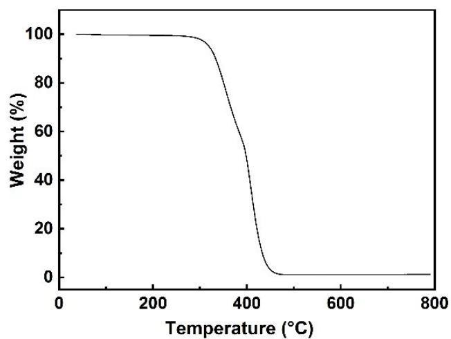
Fig. S6. TGA curve of XDI-PUE.
