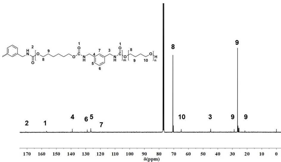
Fig. S5. ^{13}\text{C} NMR spectrum of XDI-PUE.
