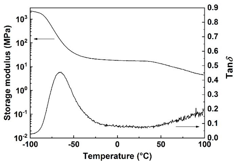
Fig. S7. DMA curve of XDI-PUE.
