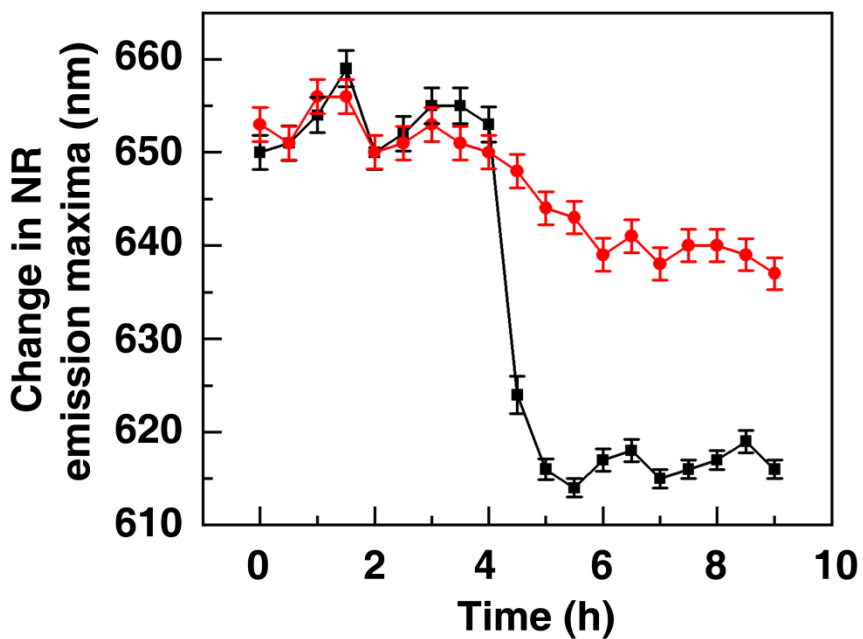
Fig. S1. Variation of the emission maxima of NR with time for HEWL samples in the absence (■) and presence (●) of COR.
