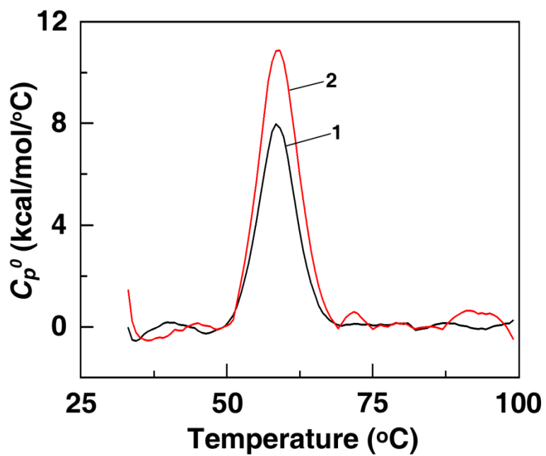
Fig. S2. DSC thermograms of HEWL (curve 1) and HEWL-COR complex (curve 2) at D/P (COR : HEWL molar ratio) = 10.
