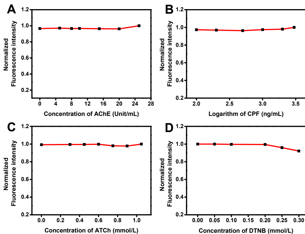
Fig. S2 The influences of individual AChE, CPF, ATCh, and DTNB on the fluorescence intensity of the CDs.
