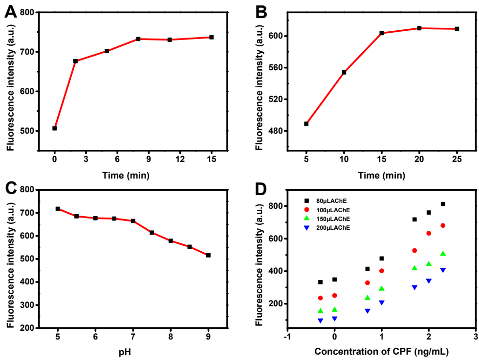
Fig. S3 The effects of (A) pre-incubation time, (B) post incubation time, (C) pH and the concentration of AChE on the fluorescence intensity of the CDs.
