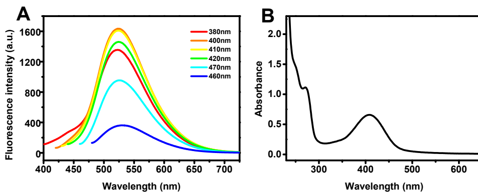
Fig. S1 (A) The emission spectra and (B) the absorption spectrum of the CDs.
