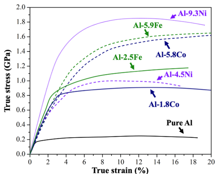
Figure S1. True stress-true strain curve associated with nanoindentation of sputtered Al-Fe, Al-Co and Al-Ni alloys.
