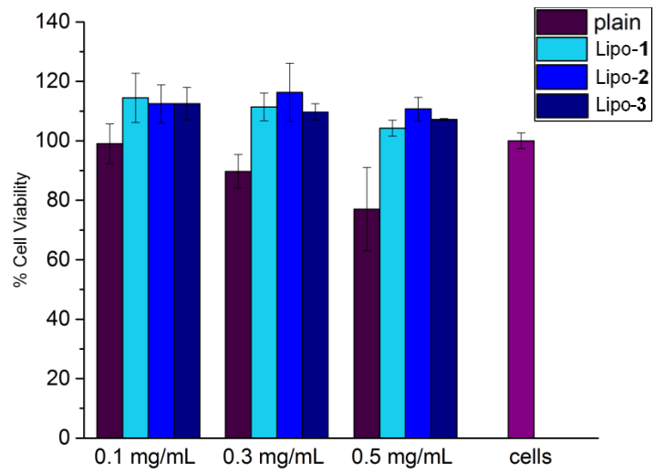
Figure S15. Cell viability in CHO-K1 cells treated with plain liposomes (purple), Lipo-1 (light blue), Lipo-2 (blue) and Lipo-3 (dark blue) after 24 hours of incubation.
