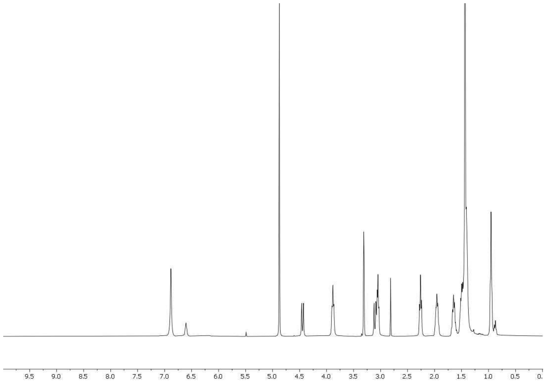
Fig. S1. ^1\text{H} NMR spectrum ( \text{CD}_3\text{OD} , 300 MHz) of compound 4.
