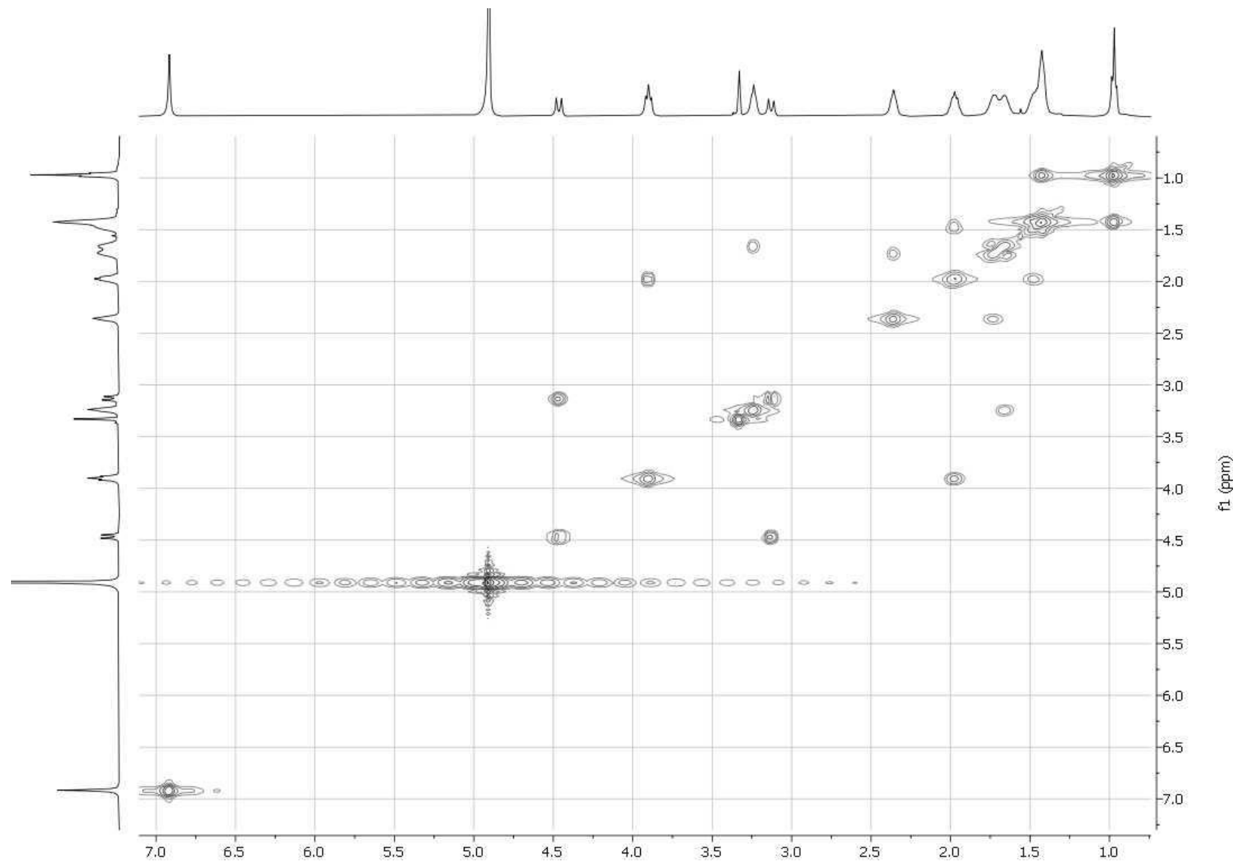
Fig. S11. ^1\text{H} COSY NMR map (400 MHz, \text{CD}_3\text{OD} ) of compound 2.
