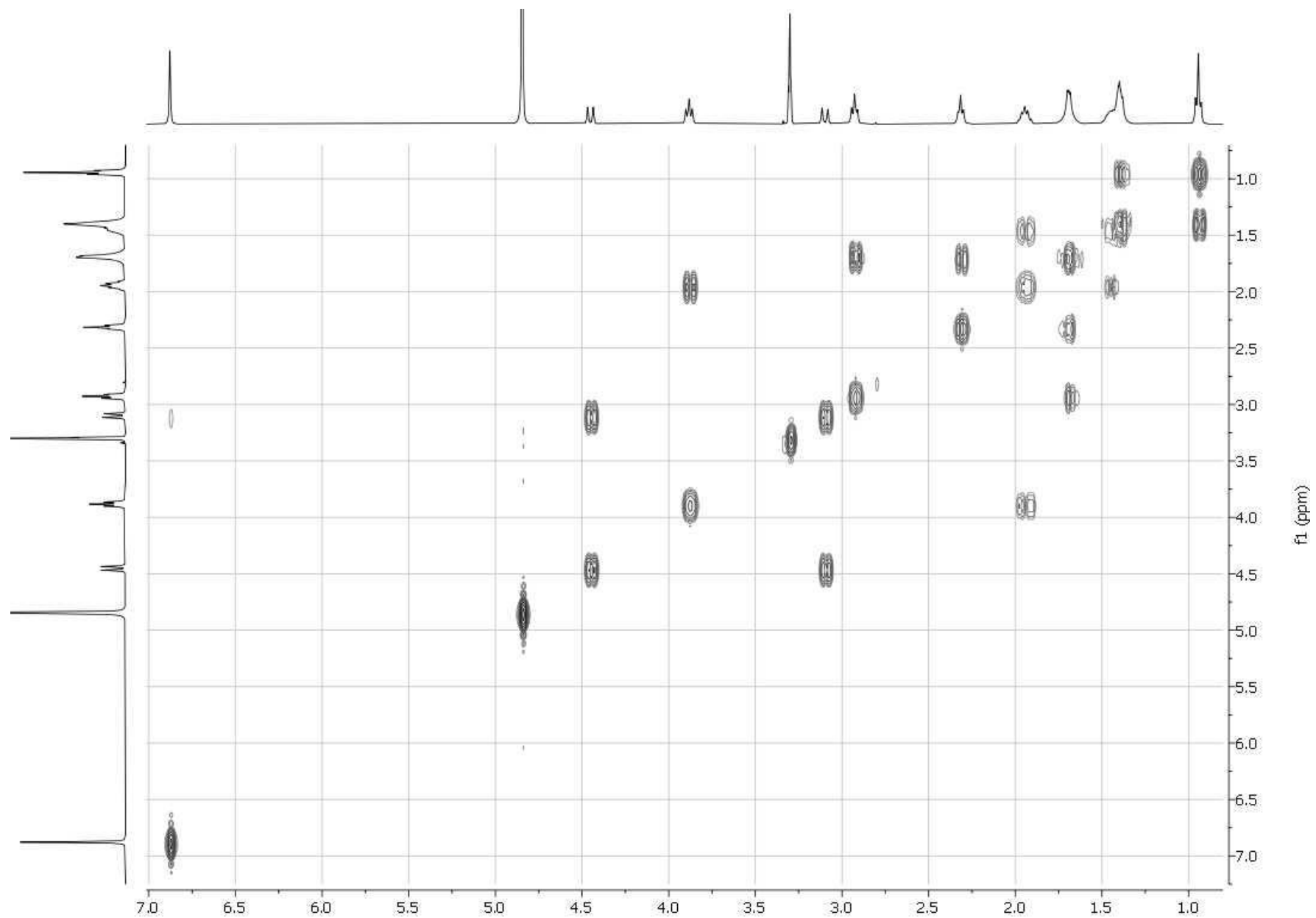
Fig. S4. 1 H COSY NMR map (400 MHz, CD 3 OD) of compound 5 .
