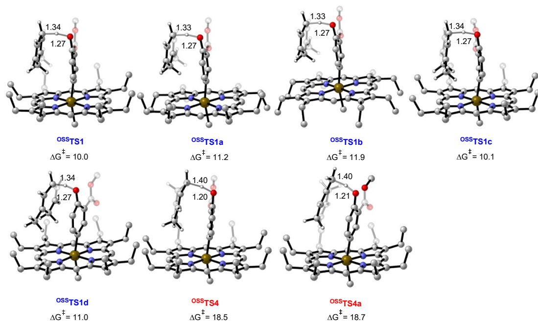
Figure S12. Different conformers for the hydrogen-atom abstraction by quinoid oxygen of the ^{OSS}Ir\text{-}QC (with substrate 1 ). The distances are shown in Å. The energies are shown in kcal mol -1 . Gibbs free energy obtained at the (U)B3LYP-D3/6-311+G(d,p)-SDD//((U)B3LYP-D3/6-31G(d)-LANL2DZ level.
