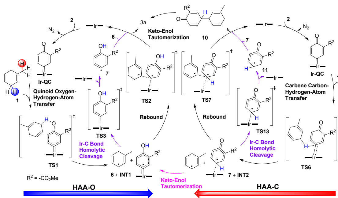
Scheme S1. Proposed catalytic cycle for Ir-porphyrin-catalyzed C–H insertion reaction of QC.
