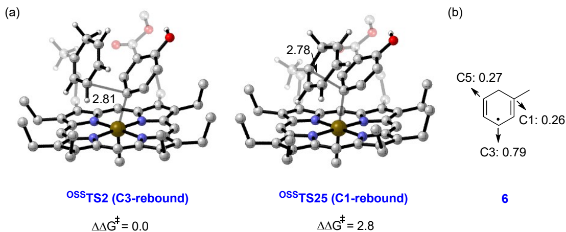
Figure S10. (a) Optimized geometries of transition states ^{OSS}TS2 and ^{OSS}TS25 . (b) Populations of spin densities for radical intermediate 6 . Hydrogen atoms on the catalyst are omitted for clarity. The distances are in Å, and energies are shown in kcal mol -1 .
