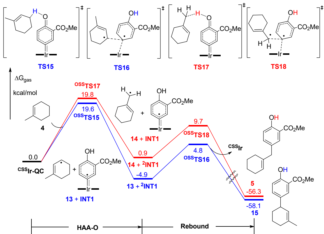
Figure S3. Gibbs free energy profiles for HAA-O catalytic cycle of insertion reaction of ^{CSS}Ir-QC to 4 . Gibbs free energy obtained at the (U)M06/6-311+G(d,p)-SDD// (U)M06/6-31G(d)-LANL2DZ level.
