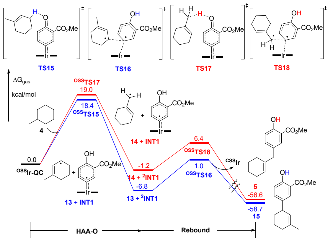
Figure S7. Gibbs free energy profiles for HAA-O catalytic cycle of insertion reaction of \text{OSSIr-QC} to 4 . Gibbs free energy obtained at the (U)MN15/6-311+G(d,p)-SDD/(U)MN15/6-31G(d)-LANL2DZ level.
