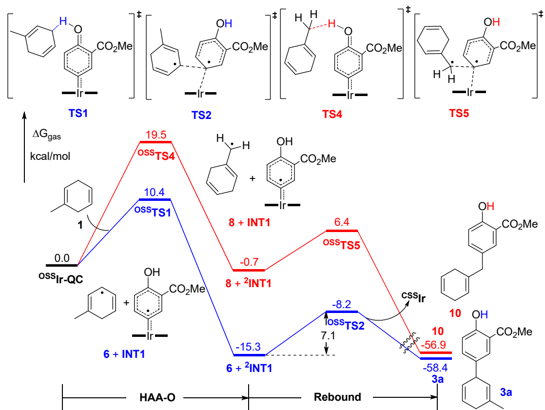
Figure S5. Gibbs free energy profiles for HAA-O catalytic cycle of insertion reaction of ^{OSS}Ir\text{-}QC to 1 . CSS is closed-shell singlet and OSS is open-shell singlet. Gibbs free energy obtained at the (U)MN15/6-311+G(d,p)-SDD//((U)MN15/6-31G(d)-LANL2DZ level.
