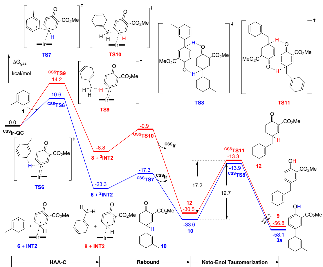
Figure S2. Gibbs free energy profiles for HAA-C catalytic cycle of insertion reaction of \text{CSSIr-QC} to 1 . The free energy of \text{CSSTS8} is given with respect to 10 , and \text{CSSTS11} is given with respect to 12 . Gibbs free energy obtained at the (U)M06/6-311+G(d,p)-SDD/(U)M06/6-31G(d)-LANL2DZ level.
