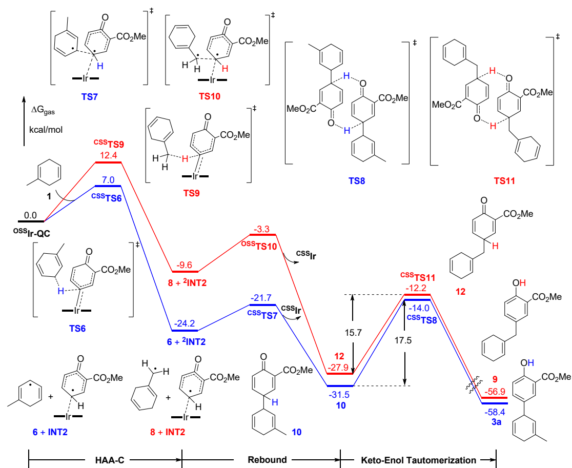
Figure S6. Gibbs free energy profiles for HAA-C catalytic cycle of insertion reaction of {}^{\text{OSS}}\text{Ir-QC} to 1 . The free energy of {}^{\text{CSS}}\text{TS8} is given with respect to 10 , and {}^{\text{CSS}}\text{TS11} is given with respect to 12 . Gibbs free energy obtained at the (U)MN15/6-311+G(d,p)-SDD//((U)MN15/6-31G(d)-LANL2DZ level.
