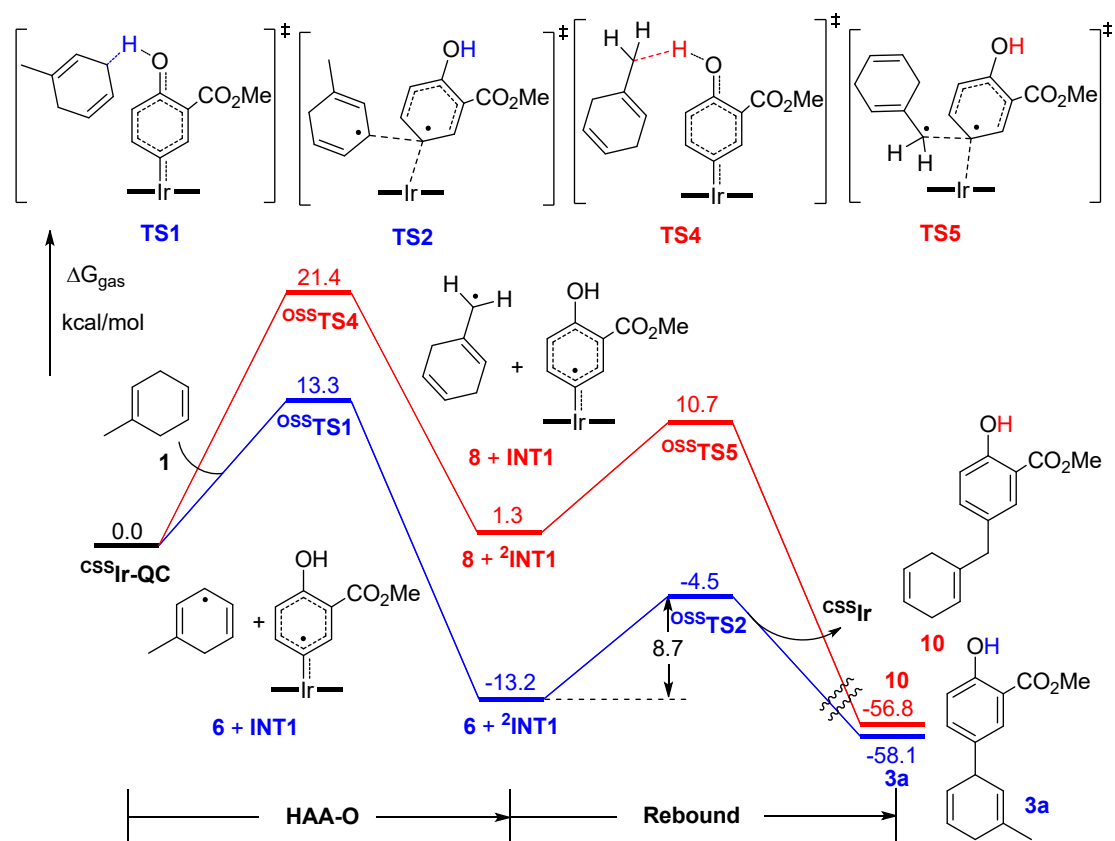
Figure S1. Gibbs free energy profiles for HAA-O catalytic cycle of insertion reaction of \text{CSSIr-QC} to 1 . CSS is closed-shell singlet and OSS is open-shell singlet. Gibbs free energy obtained at the (U)M06/6-311+G(d,p)-SDD/(U)M06/6-31G(d)-LANL2DZ level.
