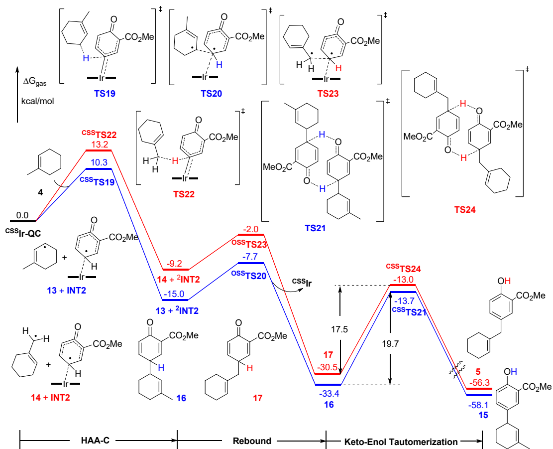
Figure S4. Gibbs free energy profiles for HAA-C catalytic cycle of insertion reaction of \text{CSSIr-QC} to 4 . The free energy of \text{CSS}^{\ddagger}\text{TS21} is given with respect to 16 and \text{CSS}^{\ddagger}\text{TS24} is given with respect to 17 . Gibbs free energy obtained at the (U)M06/6-311+G(d,p)-SDD/(U)M06/6-31G(d)-LANL2DZ level. \text{OSS}^{\ddagger}\text{TS23} were subjected to a loose convergence threshold.
