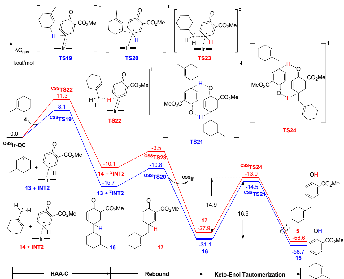
Figure S8. Gibbs free energy profiles for HAA-C catalytic cycle of insertion reaction of \text{OSSIr-QC} to 4 . The free energy of \text{CSS}^{\dagger}\text{TS21} is given with respect to 16 and \text{CSS}^{\dagger}\text{TS24} is given with respect to 17 . Gibbs free energy obtained at the (U)MN15/6-311+G(d,p)-SDD//((U)MN15/6-31G(d)-LANL2DZ level.
