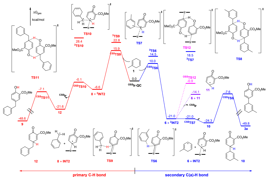
Figure S11. Gibbs free energy profiles for HAA-C catalytic cycle of insertion reaction of ^{OSS}Ir\text{-}QC to 1 . The free energy of ^{CSS}TS8 is given with respect to 10 , and ^{CSS}TS11 is given with respect to 12 . Gibbs free energy obtained at the (U)B3LYP-D3/6-311+G(d,p)-SDD//((U)B3LYP-D3/6-31G(d)-LANL2DZ level.
