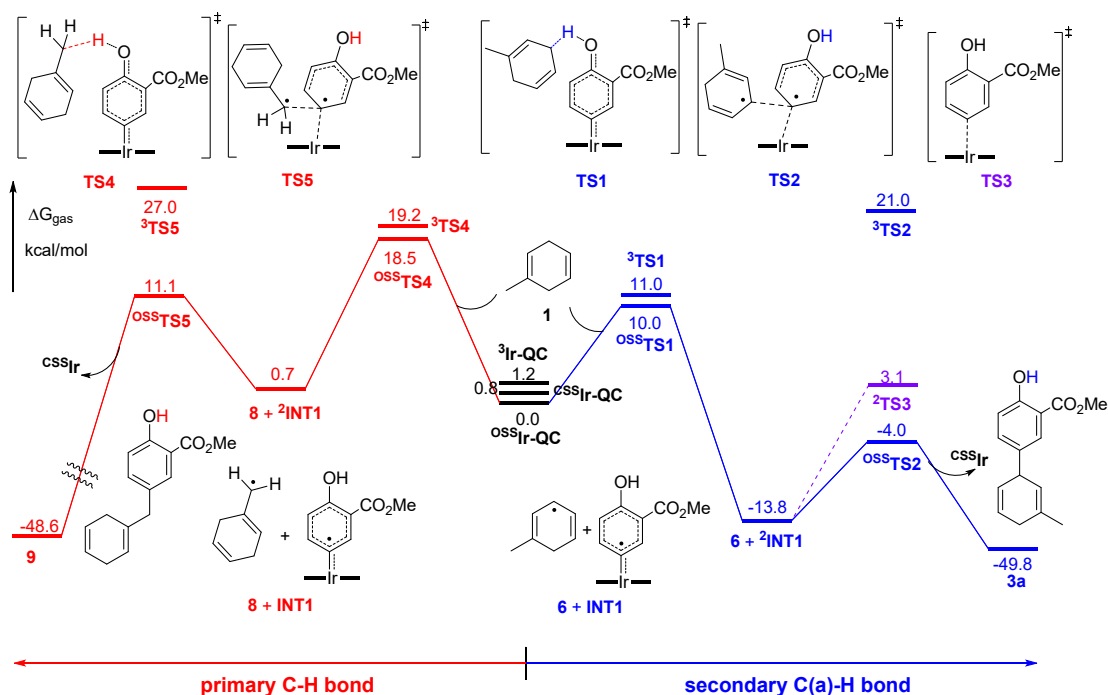
Figure S9. Gibbs free energy profiles for HAA-O catalytic cycle of insertion reaction of ^{OSS}Ir -QC to 1 . Gibbs free energy obtained at the (U)B3LYP-D3/6-311+G(d,p)-SDD// (U)B3LYP-D3/6-31G(d)-LANL2DZ level.
