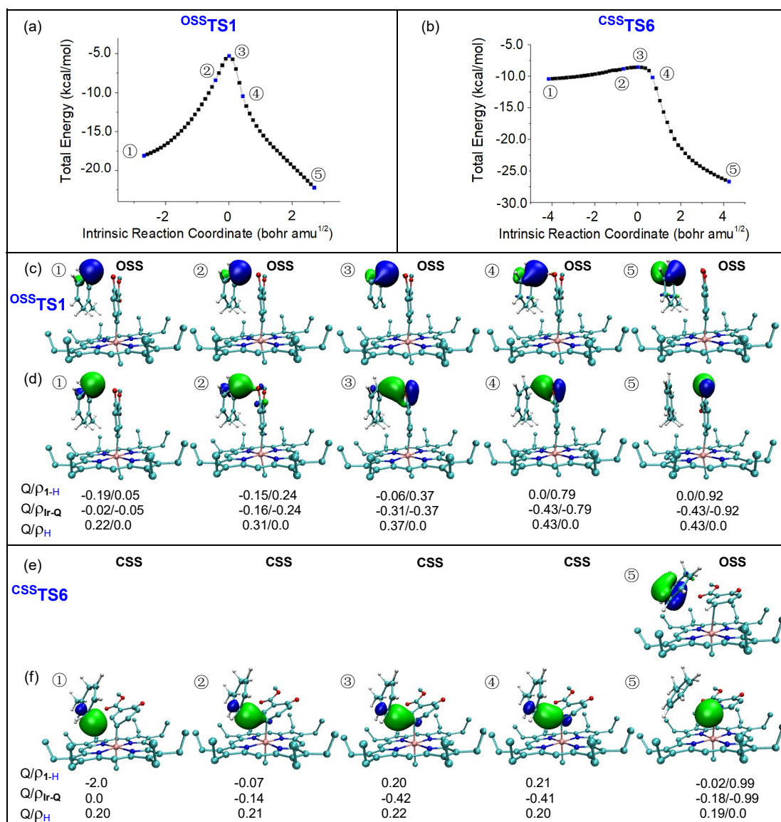
Figure S14. Plots of the change in electronic energies along the intrinsic reaction coordinate (IRC) for oss TSS1 (a) and css TSS6 (b). (c) α-LMOs and (d) β-LMO analysis along the IRC between quinoid oxygen of the Ir-QC and 1 , and the Mulliken charges (Q) and spin densities (ρ) on the hydrogen-atom abstracted moieties (1-H) and on the Ir-QC. (e) α-LMOs and (f) LMO analysis along the IRC between carbene carbon of the Ir-QC and 1 , and the Mulliken charges (Q) and spin densities (ρ) on the hydrogen-atom abstracted moieties (1-H) and on the Ir-QC.
